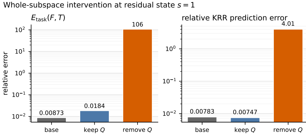
Figure 7: Experiment 3 whole-subspace complement ablation at s = 1 . Left: task finite-difference operator error E_{\text{task}}(F, T) after no surgery, keep- Q , and remove- Q . Right: relative pointwise KRR prediction error for the same three interventions. Keeping only P_Q^A H_s^{\text{ctx}} nearly preserves the task-local behavior; deleting it leaves the complement and destroys the KRR response.
