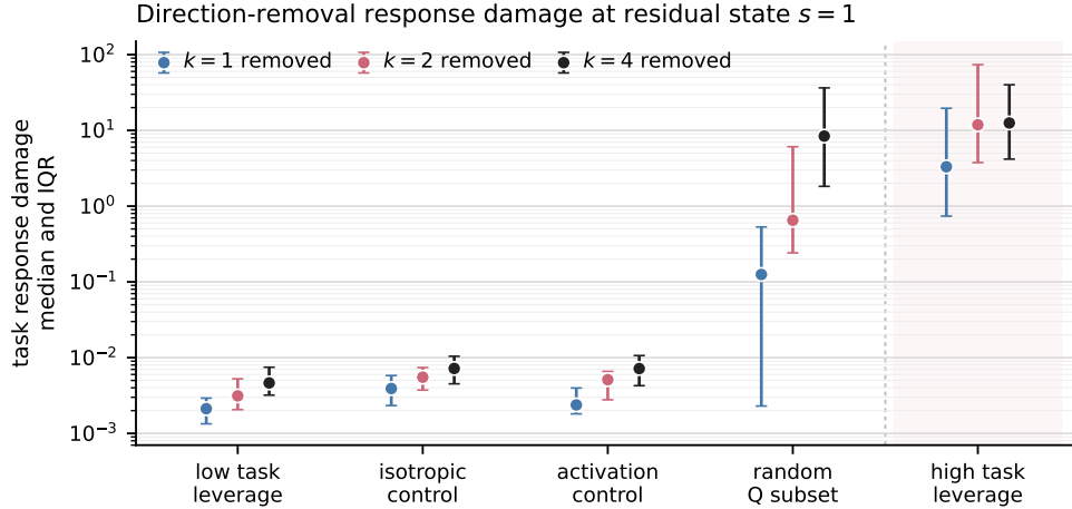
Figure 6: Experiment 3 selective causal effect. High task-leverage removals cause much larger task finite-difference response damage than matched low-task-leverage controls.
