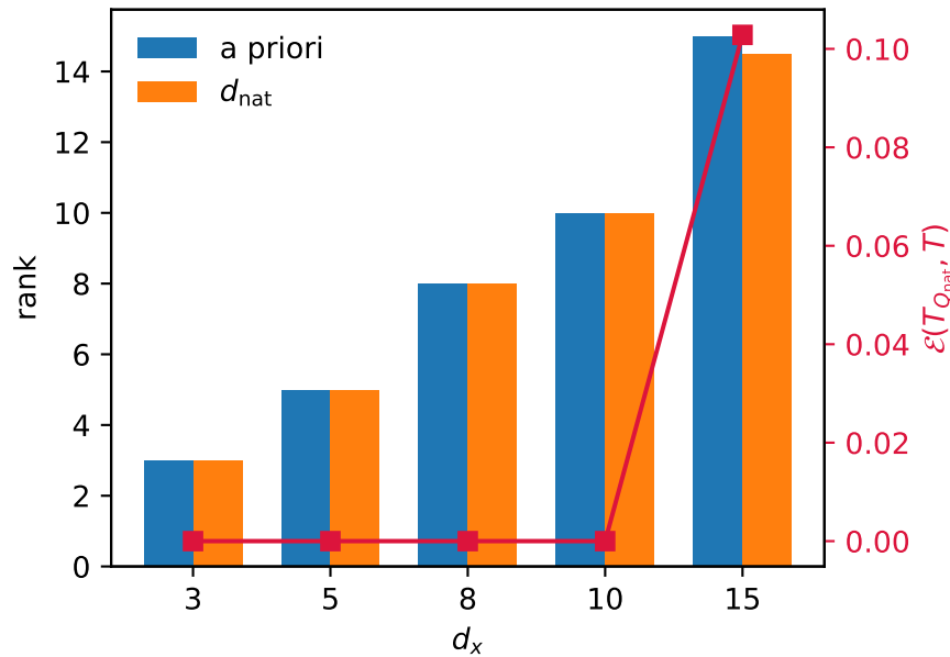
Target-rank sweep
