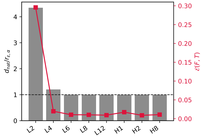
Architecture sweep
