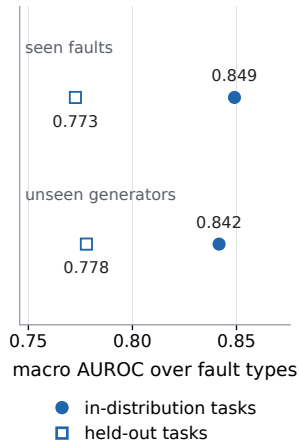
b Frozen detector, macro AUROC
