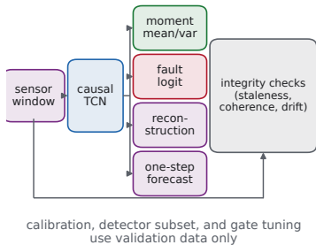
b Shared TCN and evidence heads
