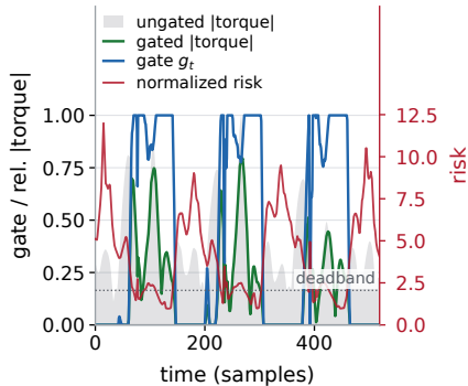
c Risk above deadband attenuates
