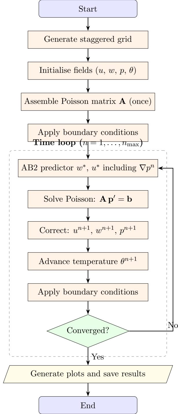
Figure 3: Algorithm flowchart for the pipe flow solver.
