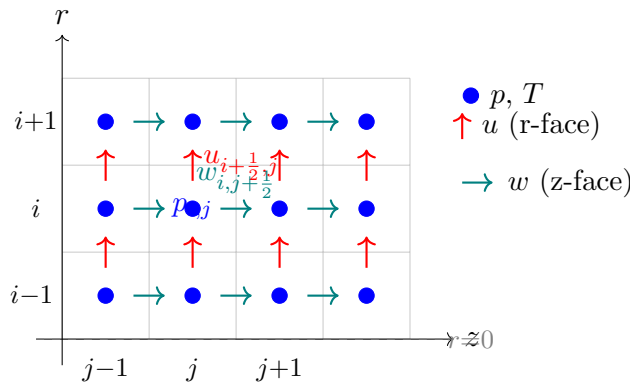
Figure 11: Staggered grid in the ( r, z ) plane. Scalars ( p, T ) at cell centres (blue); radial velocity u on horizontal faces (red); axial velocity w on vertical faces (teal). The dashed line marks the symmetry axis r = 0 .
