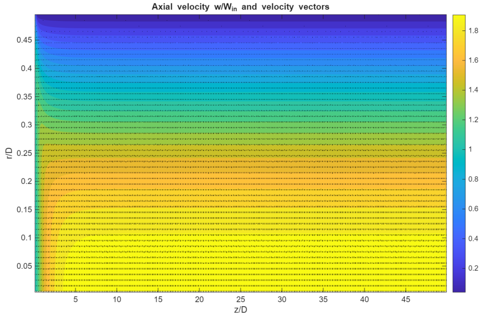
Figure 5: Axial velocity contour w/W_{\text{in}} with all cell-centre velocity vectors. The flow transitions from a uniform inlet profile ( w = 1 ) to a parabolic profile ( w_{\text{max}} = 2 at centreline); the arrows show the axial and radial components of the velocity field at every plotted cell centre.
