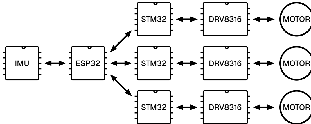
Figure 2: block diagram of the controll circuit
