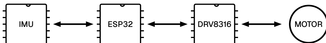
Figure 2: block diagram of the controll circuit
