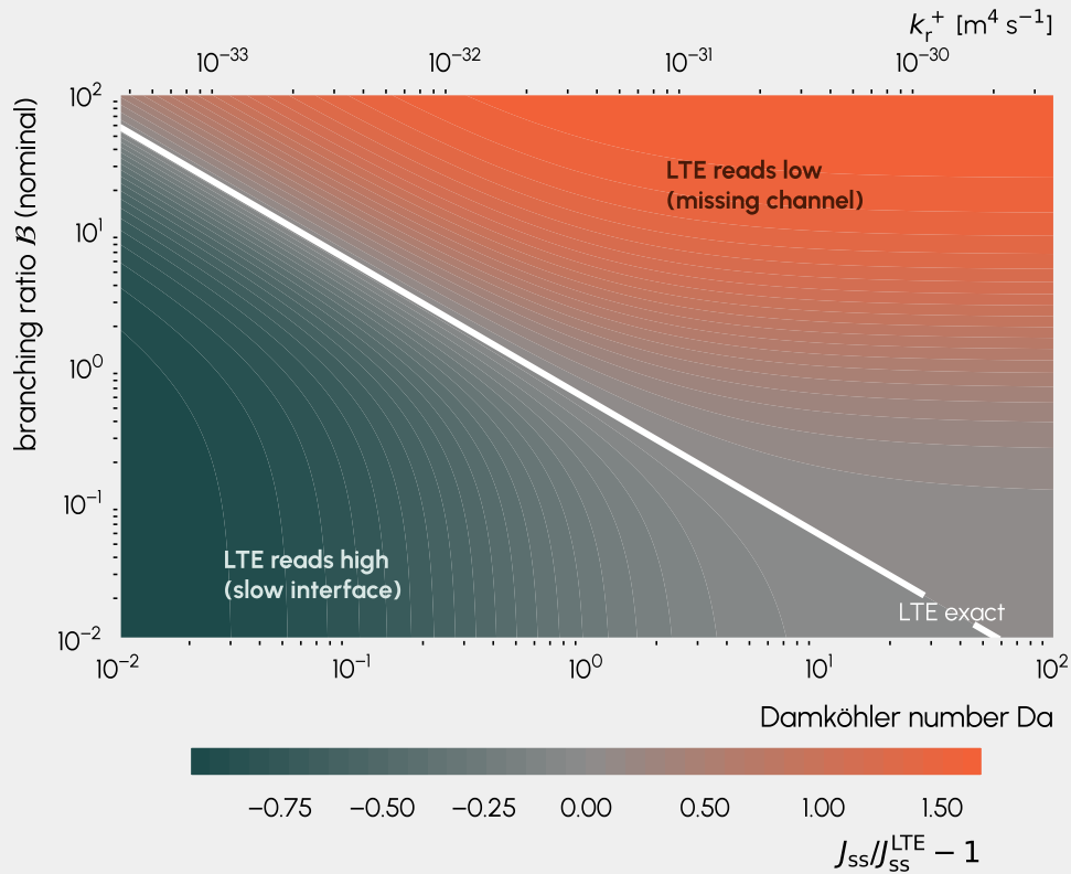
(a) steady flux, analytical solution
