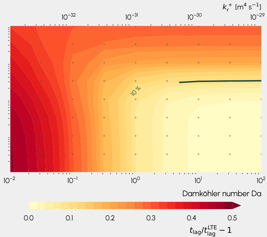
(b) time lag, 81 transient solves
