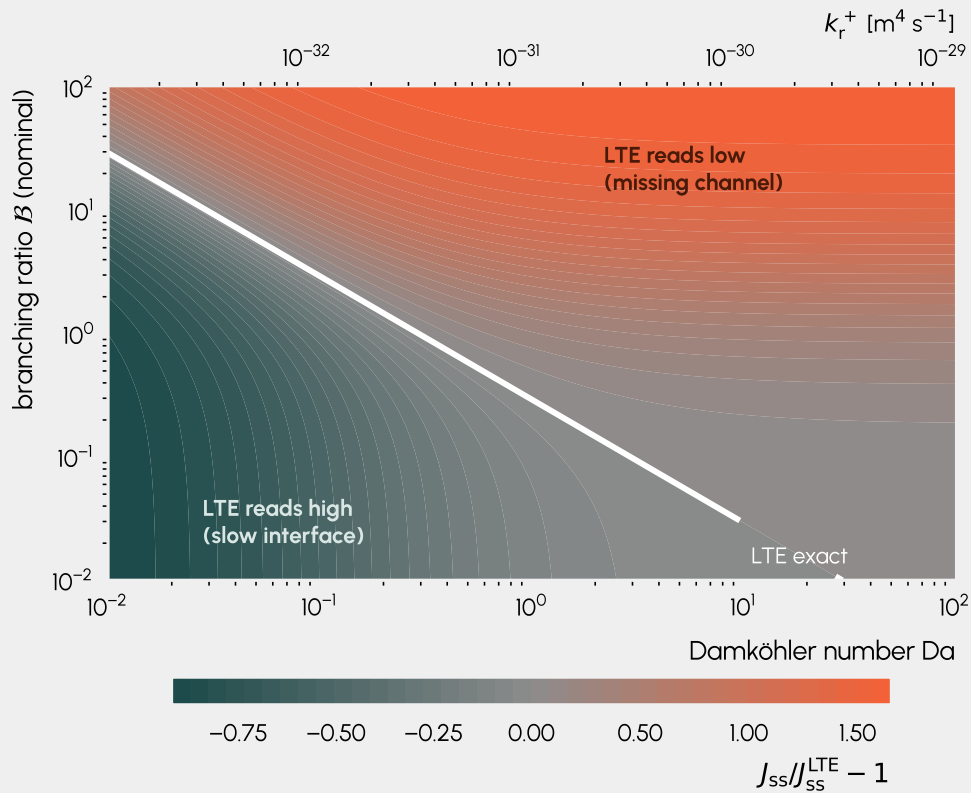
(a) steady flux, closed form
