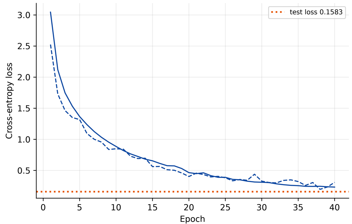
(b) Loss
