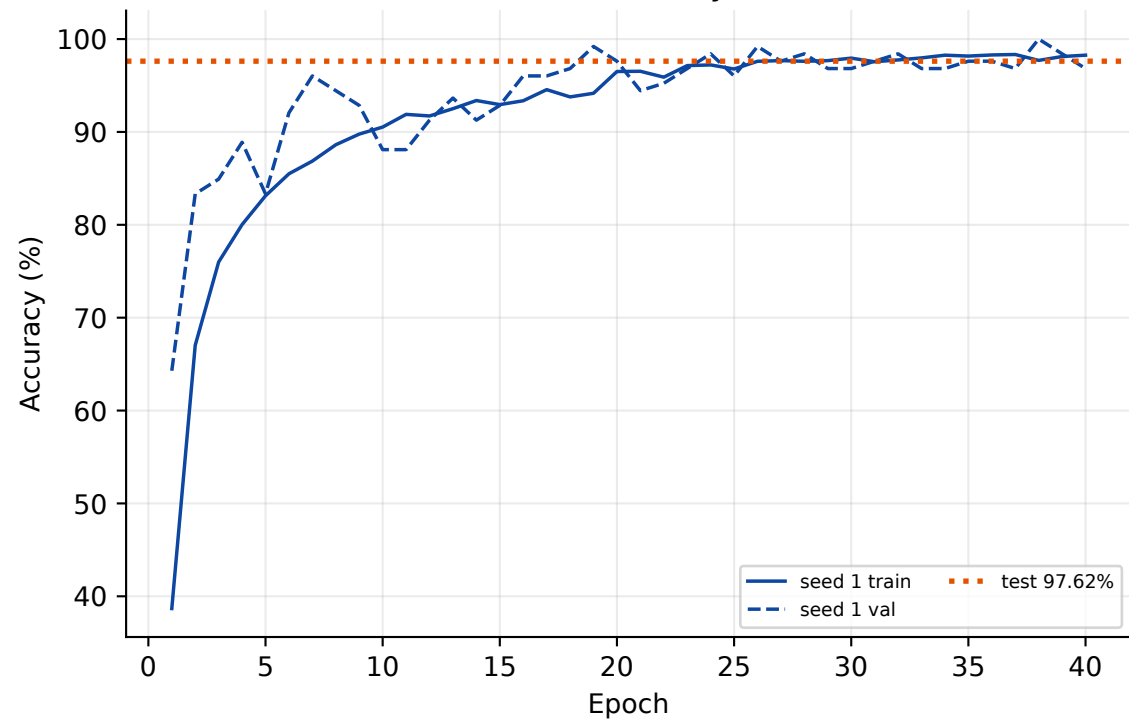
(a) Accuracy
