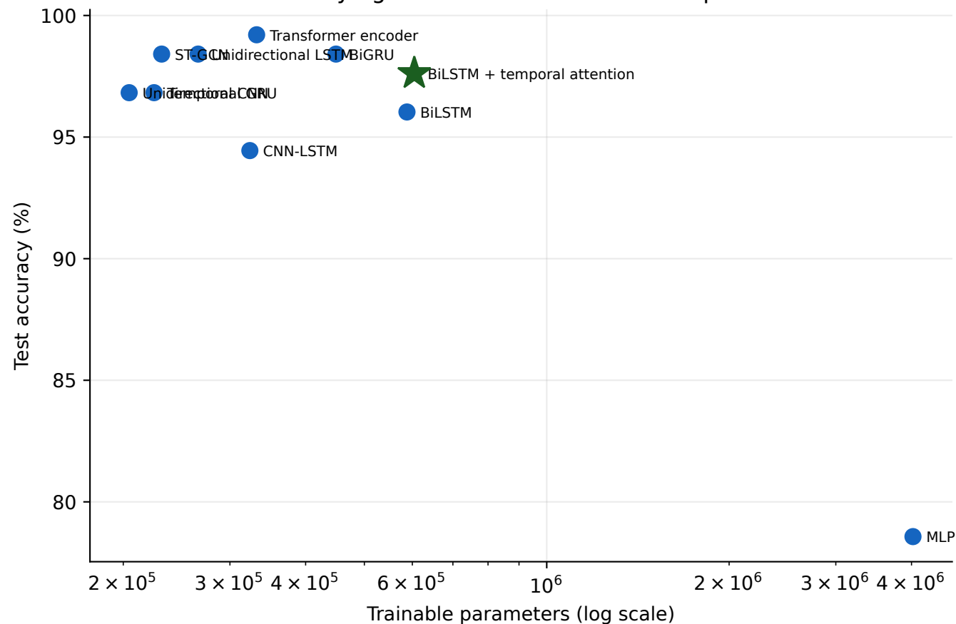
Accuracy against model size under one protocol
