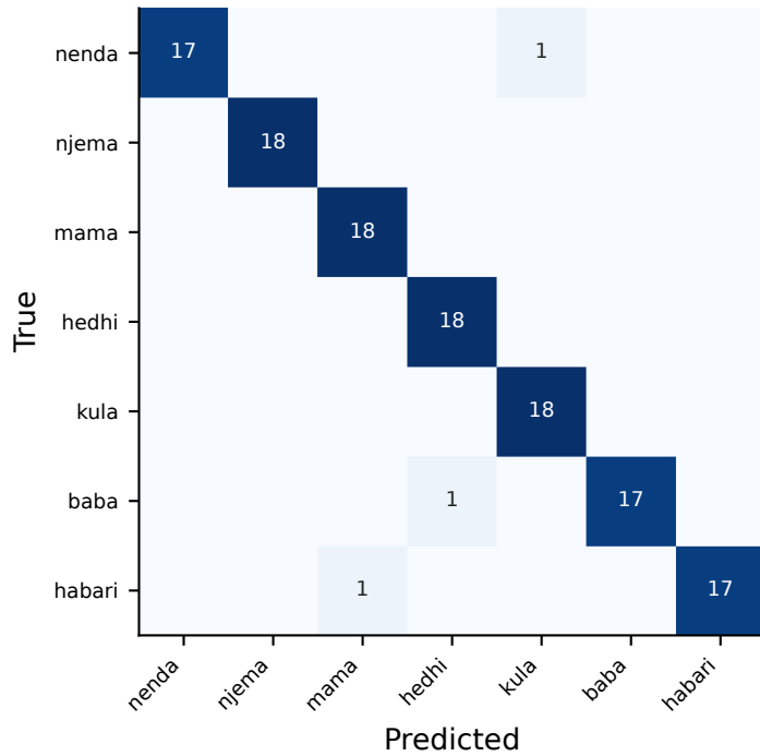
signer-dependent (reference)
