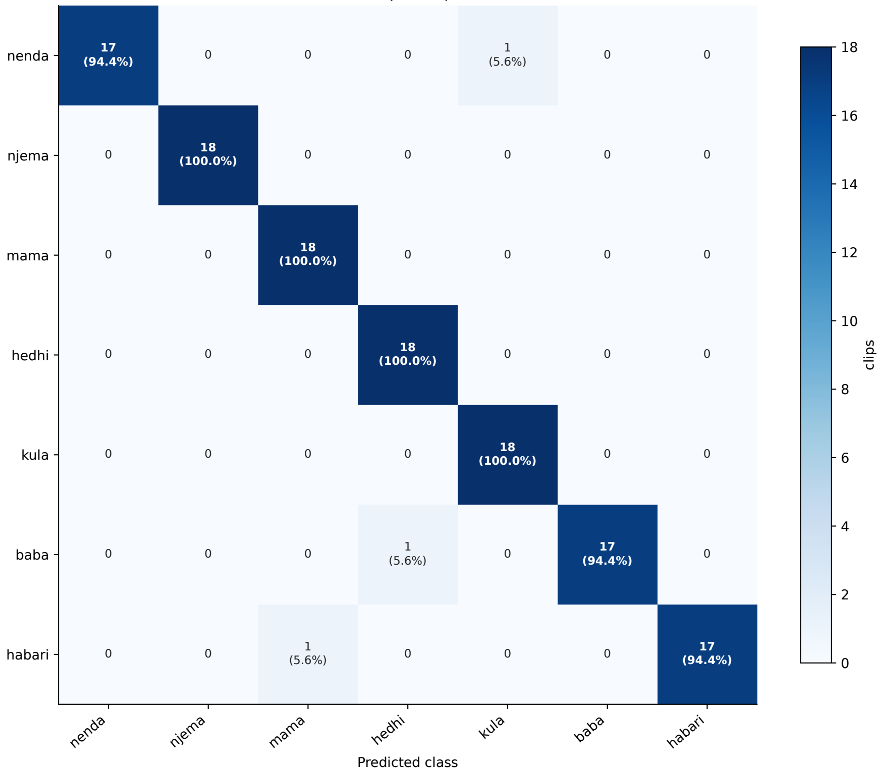
Confusion matrix: count (row percentage) 126 test clips, 18 per class
