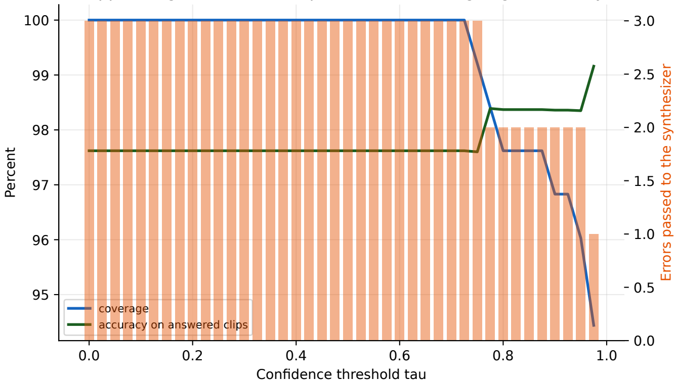
Suppressing low-confidence predictions: coverage against safety
