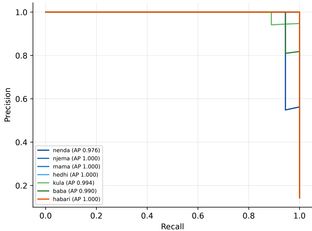
(b) Precision-recall (macro AP 0.9942)
