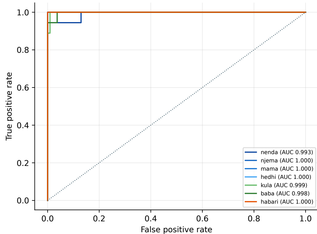
(a) ROC, one-vs-rest (macro AUC 0.9985)
