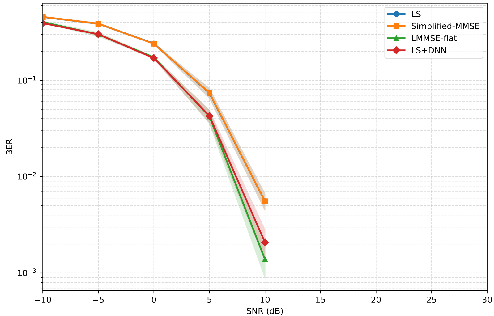
BER vs SNR — AWGN (mean \pm std, seeds [42, 123, 999])
