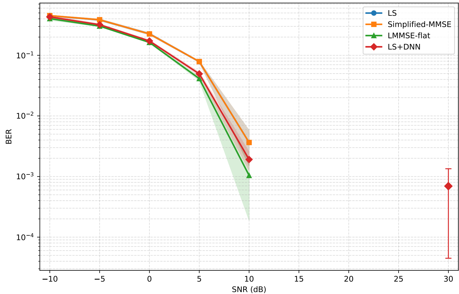
BER vs SNR — RAYLEIGH (mean \pm std, seeds [42, 123, 999])
