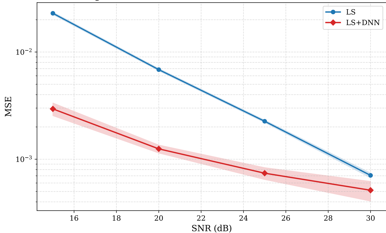
High-SNR error floor — AWGN (15-30 dB, mean \pm std)
