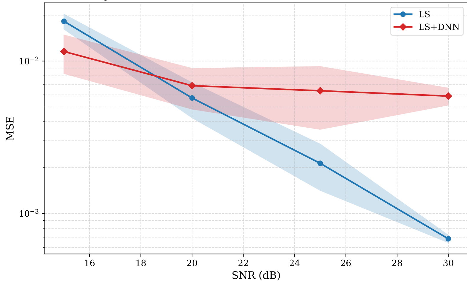
High-SNR error floor — RAYLEIGH (15–30 dB, mean \pm std)
