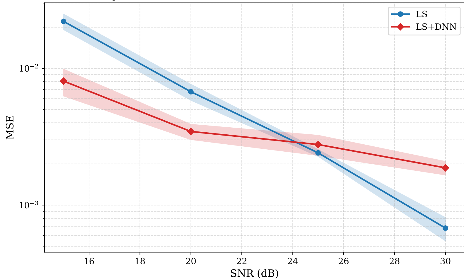
High-SNR error floor — RICIAN (15-30 dB, mean \pm std)
