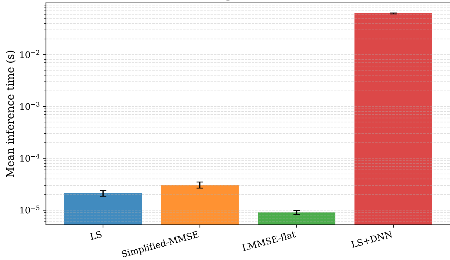
Inference time comparison (mean over 9 runs)
