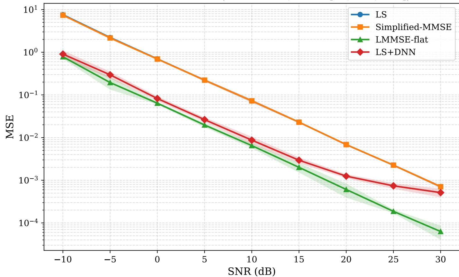
MSE vs SNR — AWGN (mean \pm std, seeds [42, 123, 999])
