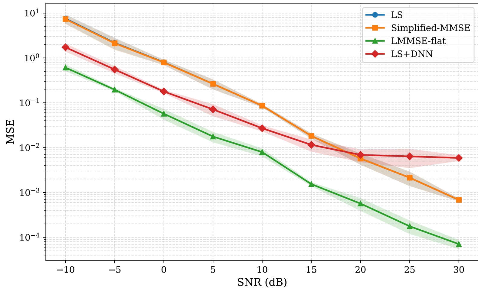
MSE vs SNR — RAYLEIGH (mean \pm std, seeds [42, 123, 999])
