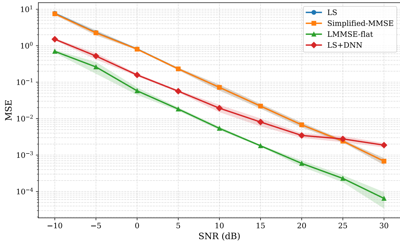
MSE vs SNR — RICIAN (mean \pm std, seeds [42, 123, 999])
