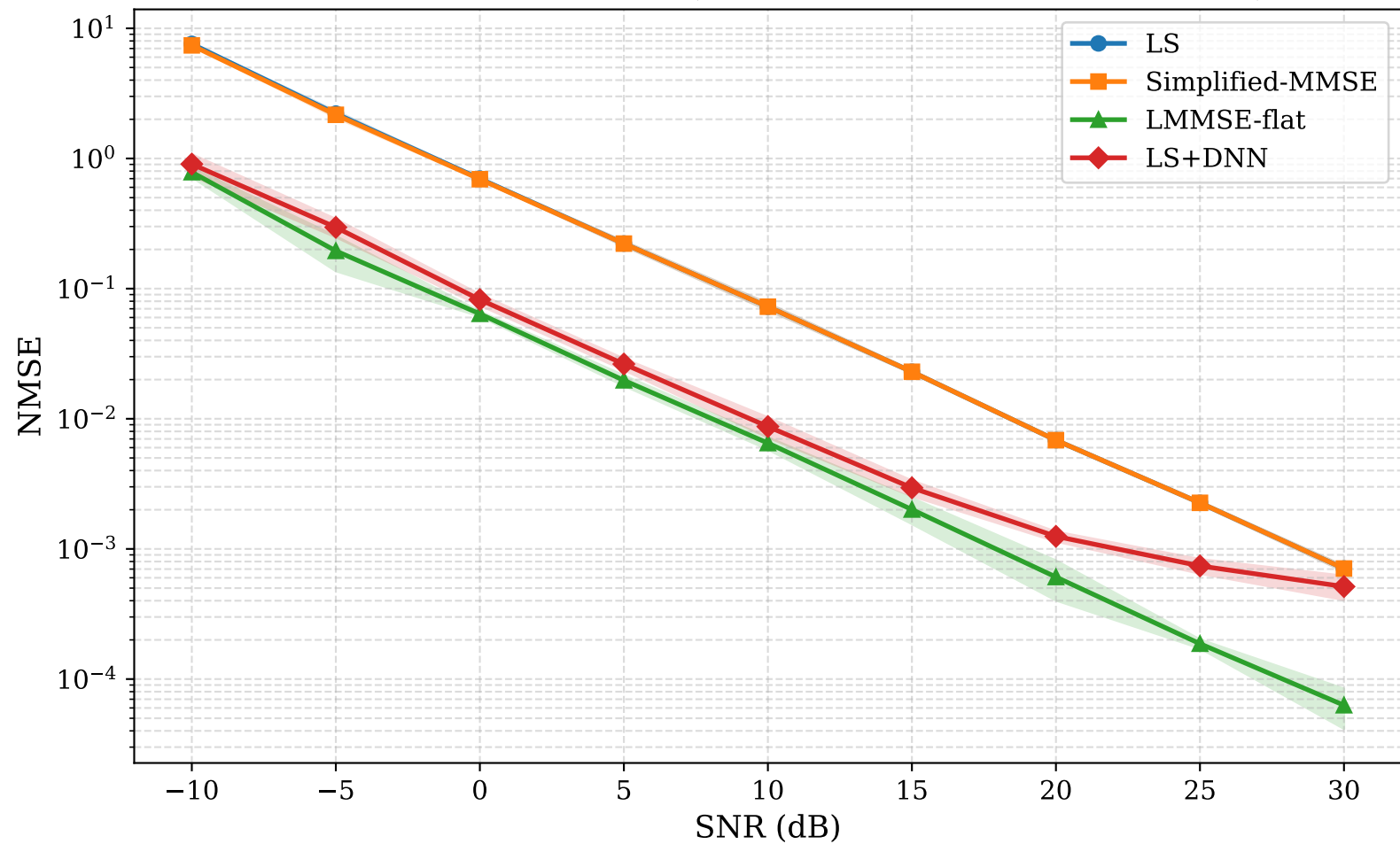
NMSE vs SNR — AWGN (mean \pm std, seeds [42, 123, 999])
