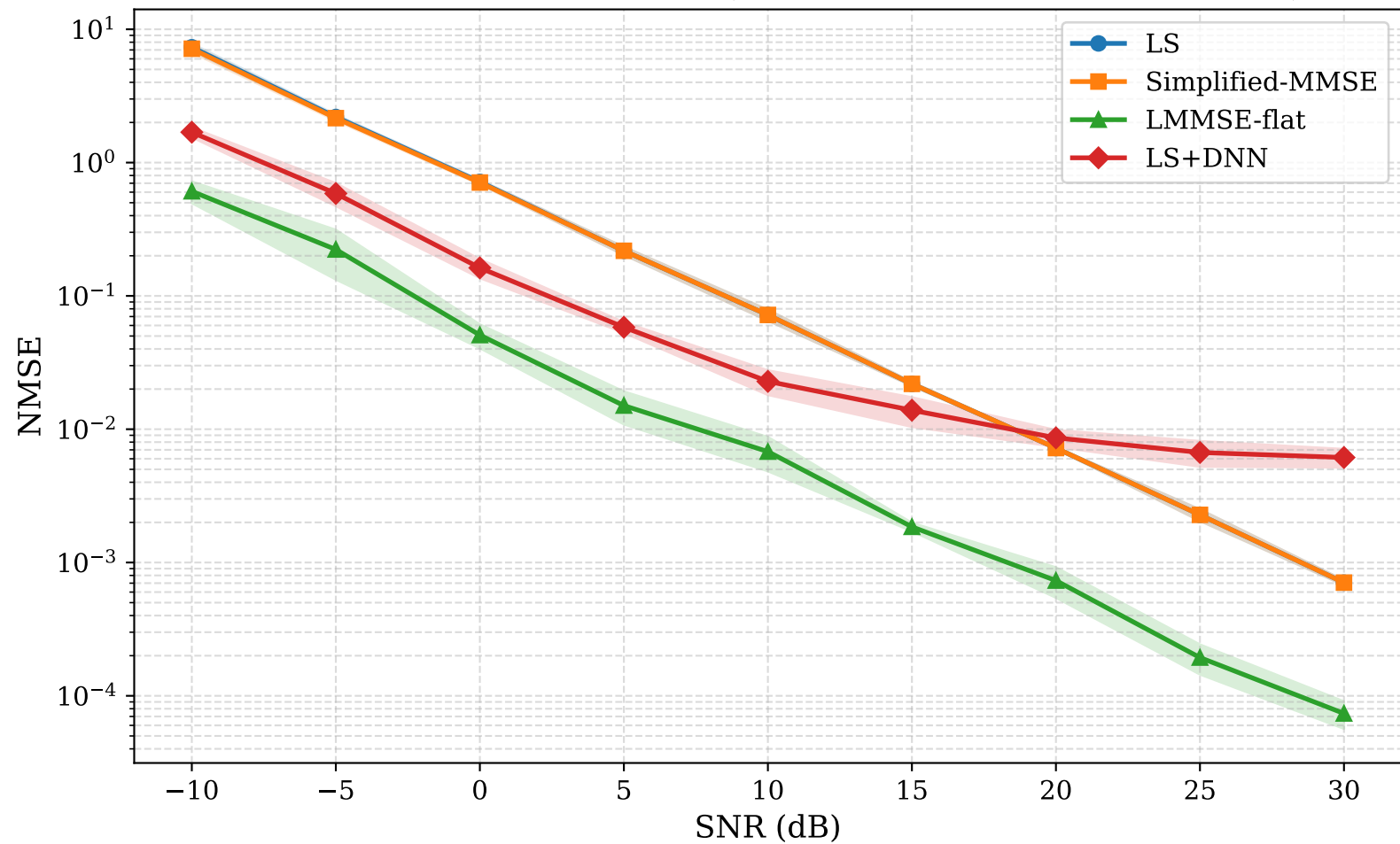
NMSE vs SNR — RAYLEIGH (mean \pm std, seeds [42, 123, 999])
