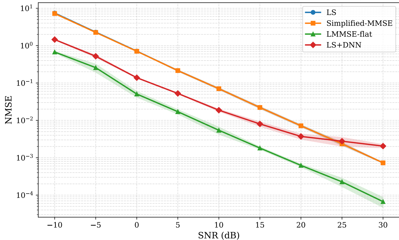
NMSE vs SNR — RICIAN (mean \pm std, seeds [42, 123, 999])
