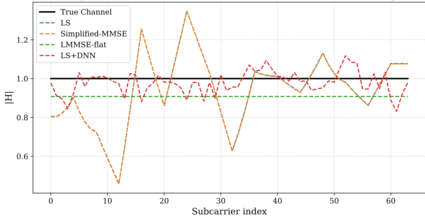
Sample channel estimate — AWGN (SNR=10 dB, seed=42, flat fading)
