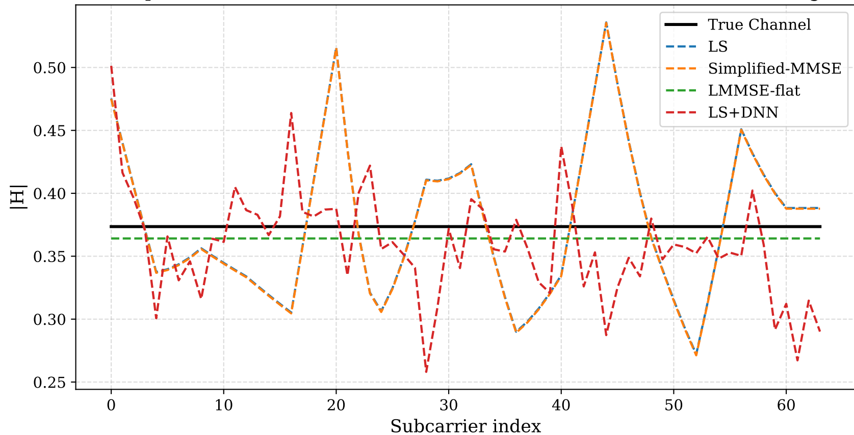
Sample channel estimate — RAYLEIGH (SNR=10 dB, seed=42, flat fading)
