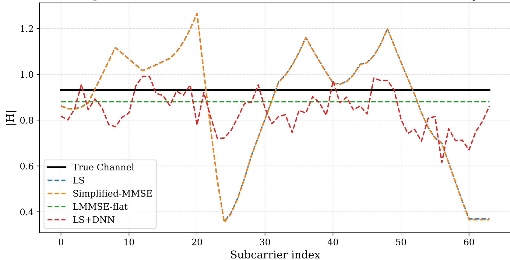
Sample channel estimate — RICIAN (SNR=10 dB, seed=42, flat fading)
