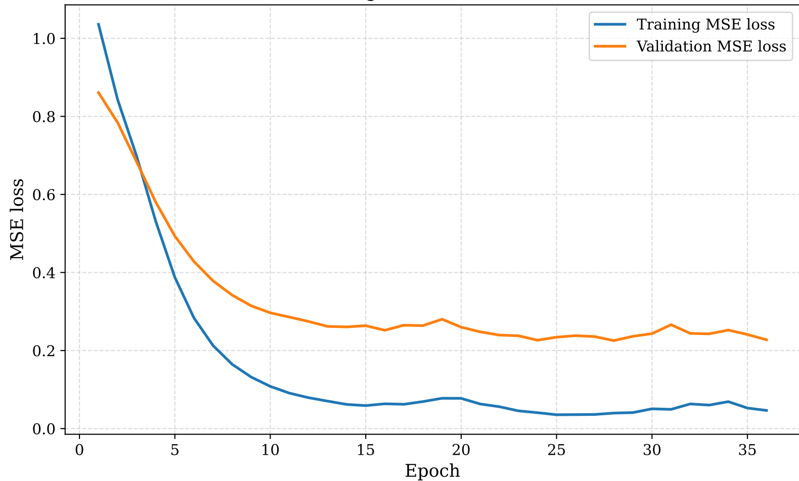
DNN training — RAYLEIGH (seed=42)
