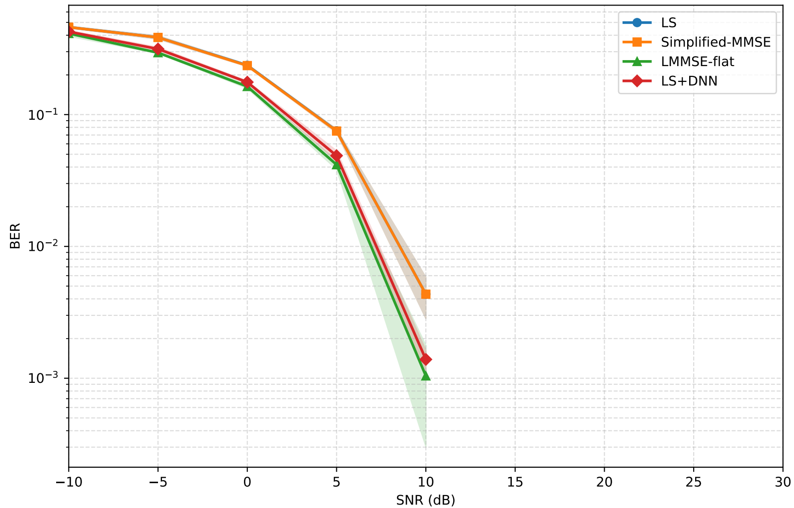
BER vs SNR — RICIAN (mean \pm std, seeds [42, 123, 999])
