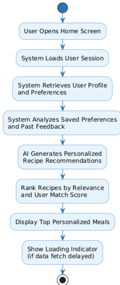
Figure 4.5-3 Activity Diagram: Meal Recommendation
