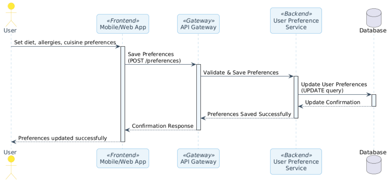
Figure 4.6-2 Sequence Diagram: User Preference
