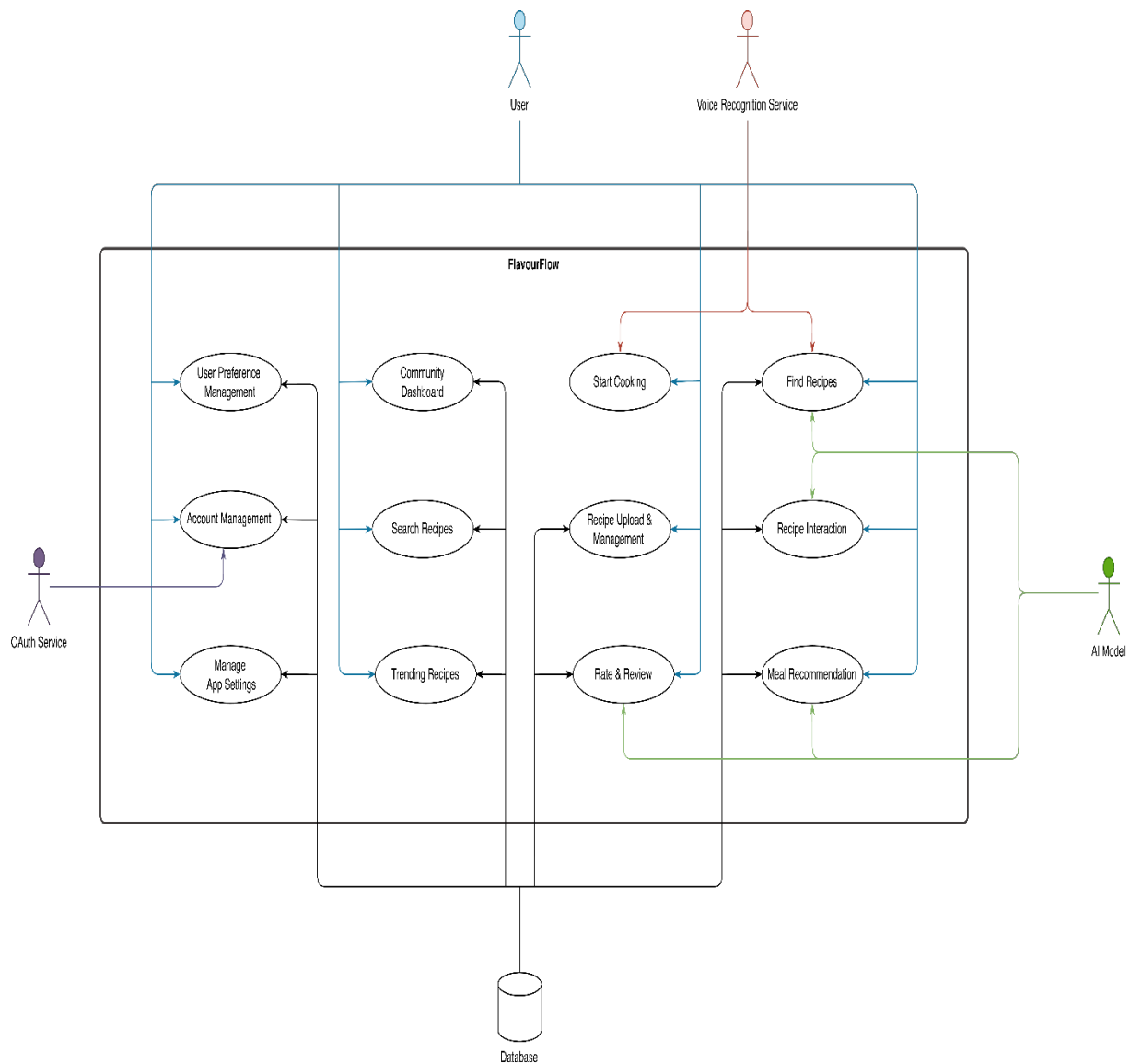
Figure 3.1-1: System Use Cases
