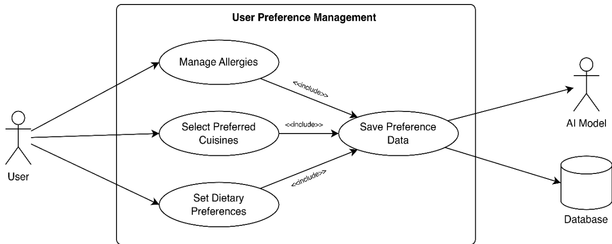
Figure 3.1-2: User Preference Management
