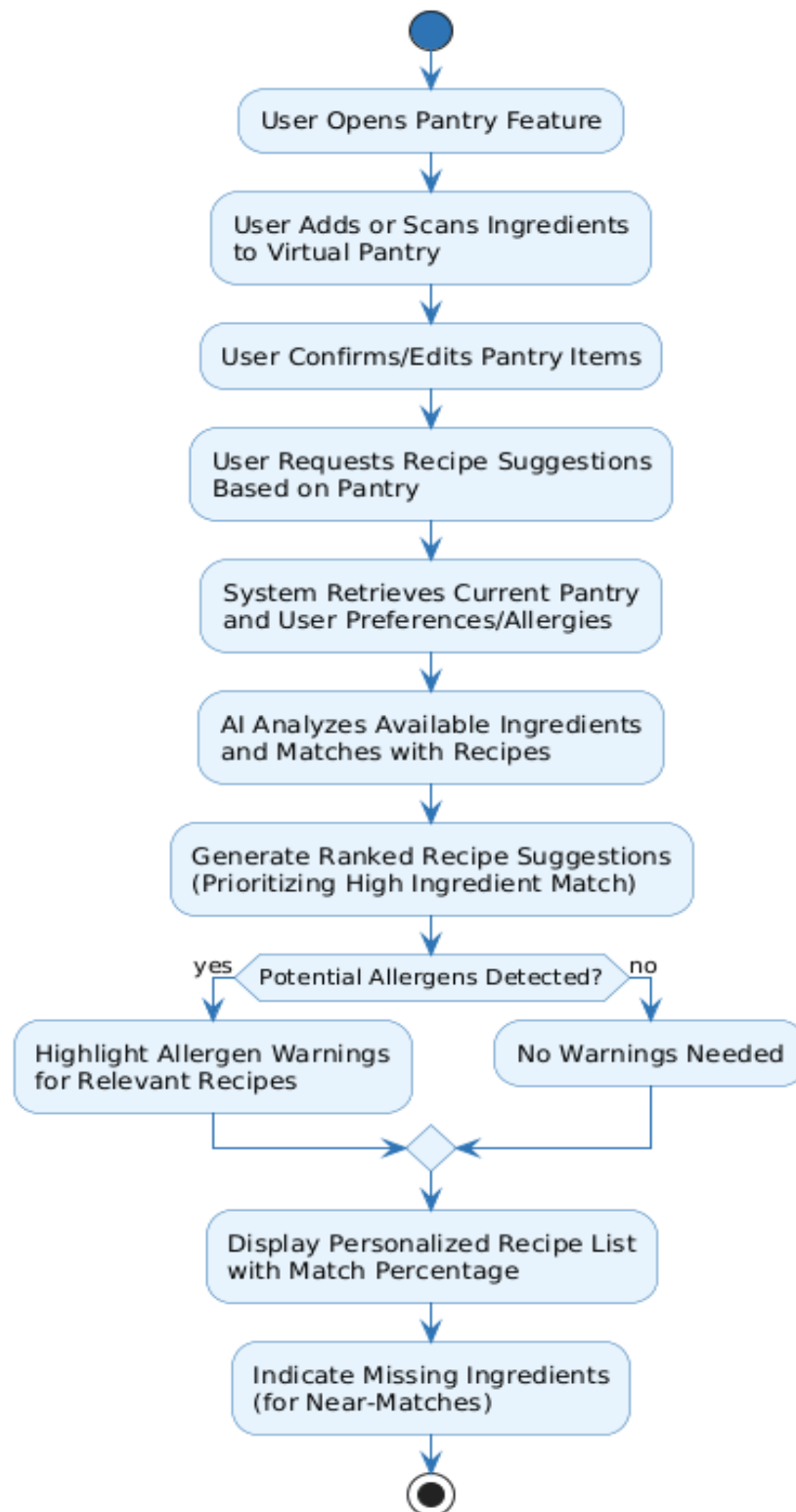
Figure 4.5-9 Activity Diagram: Smart Pantry & Ingredient Insights
