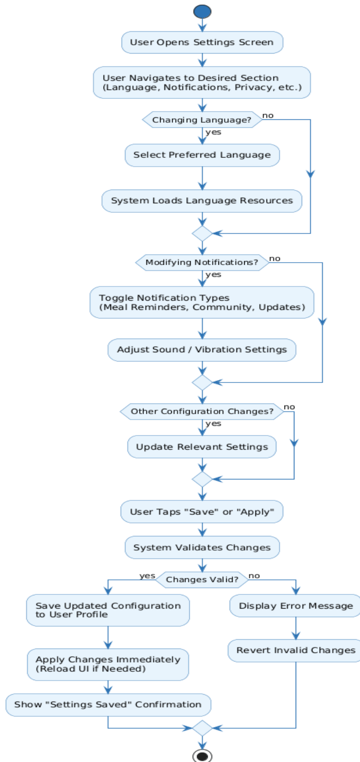
Figure 4.5-12 Activity Diagram: Manage Application Settings
