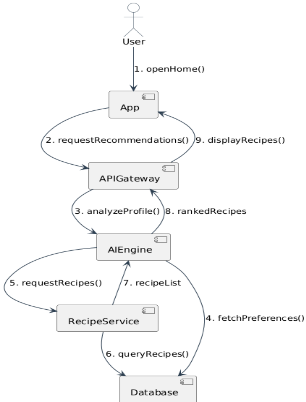
Figure 4.7-2 Collaboration Diagram: Personalized
