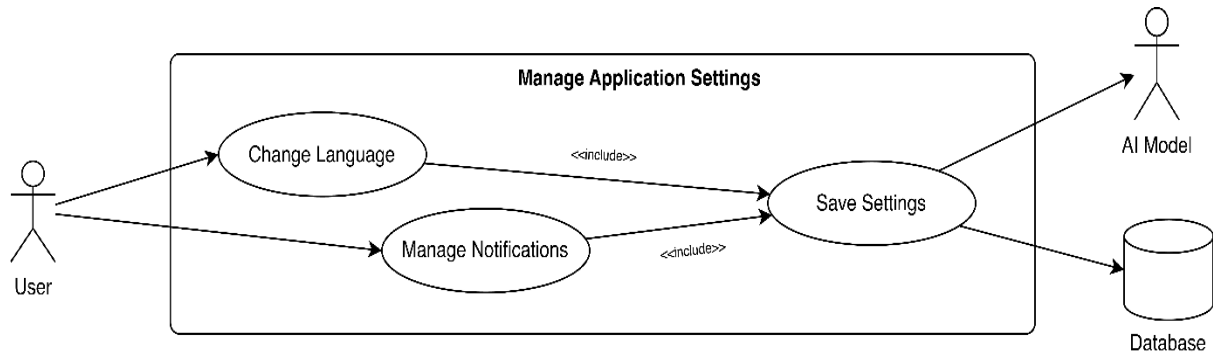
Figure 3.1-12: Manage Application Settings
