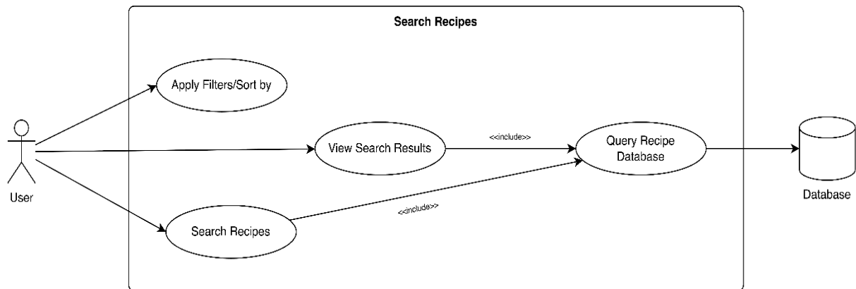
Figure 3.1-4: Search Recipes
