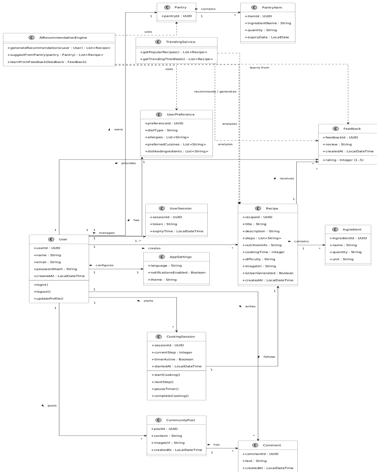
Figure 4.4-1 Class Diagram
