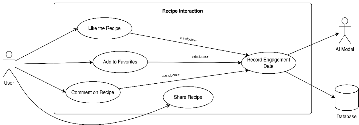
Figure 3.1-5: Recipe Interaction
