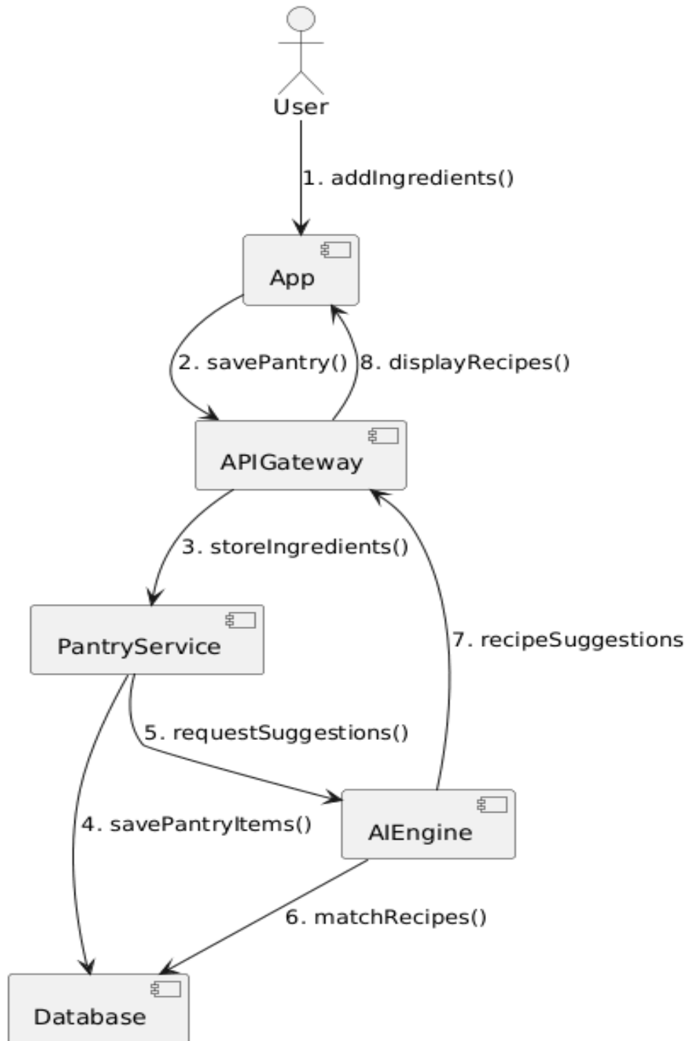
Figure 4.7-5 Collaboration Diagram: Smart Pantry
