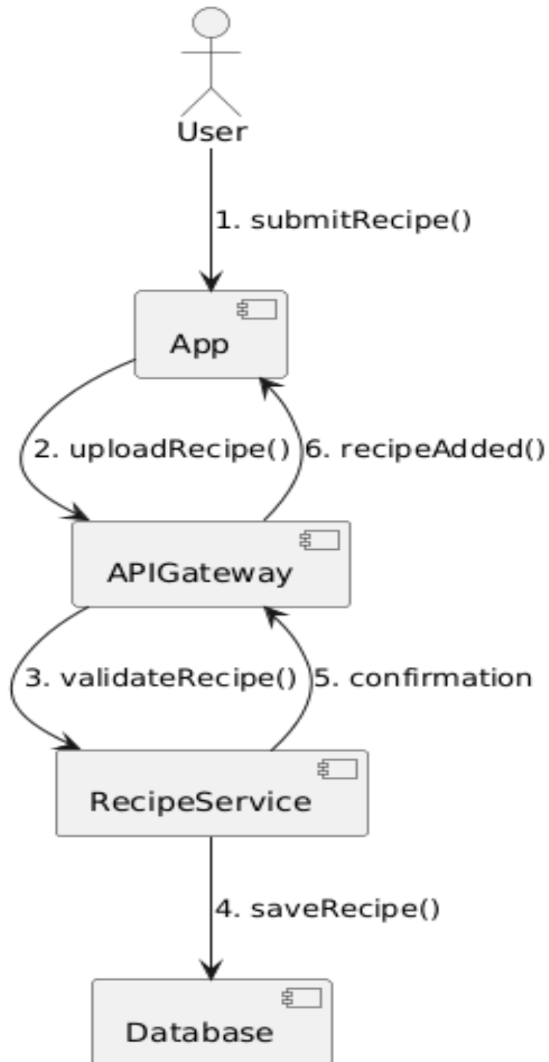
Figure 4.7-4 Collaboration Diagram: User Recipe
