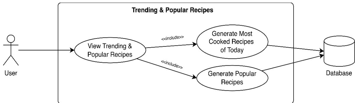
Figure 3.1-11: Trending and Popular Recipes
