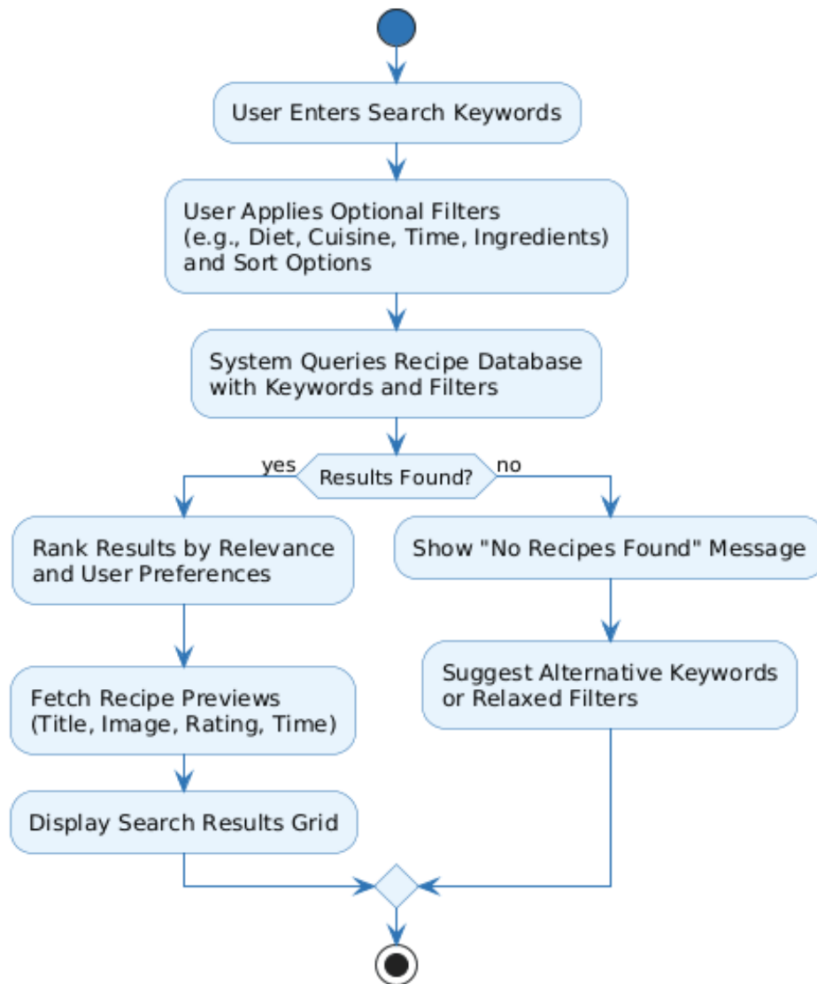
Figure 4.5-5 Activity Diagram: Recipe Search & Discovery
