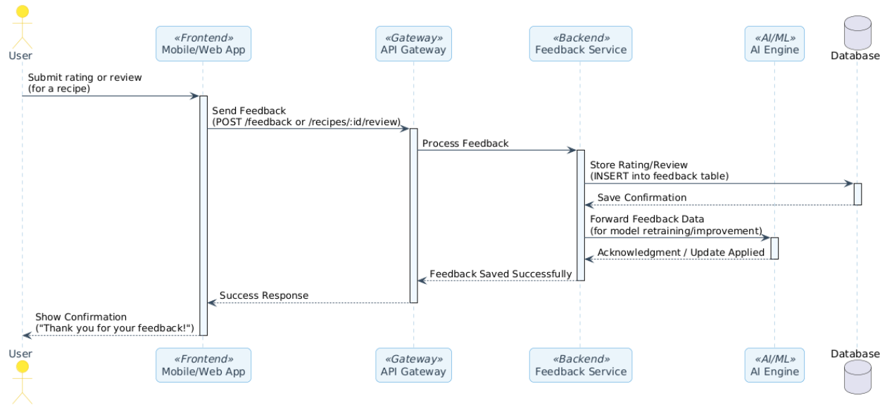
Figure 4.6-8 Sequence Diagram: Feedback & Rating
