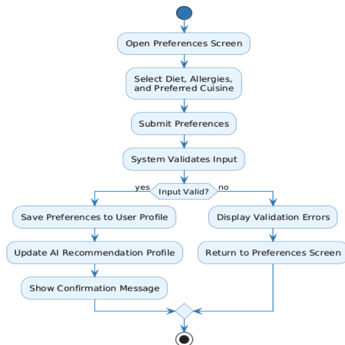
Figure 4.5-2 Activity Diagram: User Preference
