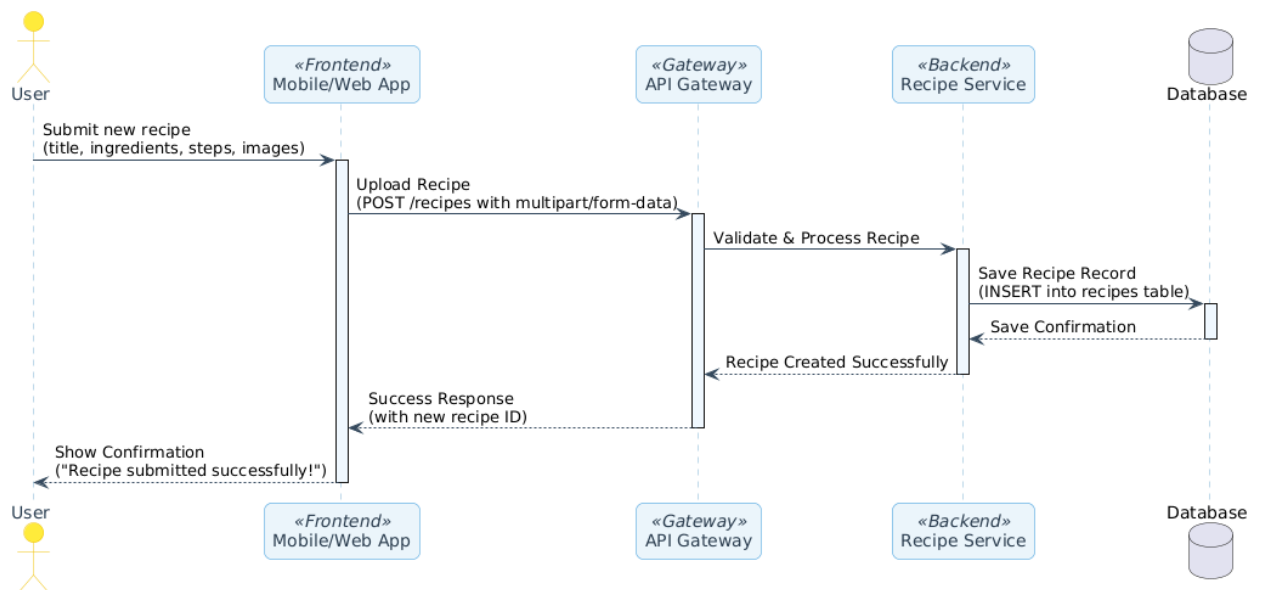
Figure 4.6-7 Sequence Diagram: Recipe Upload & Management
