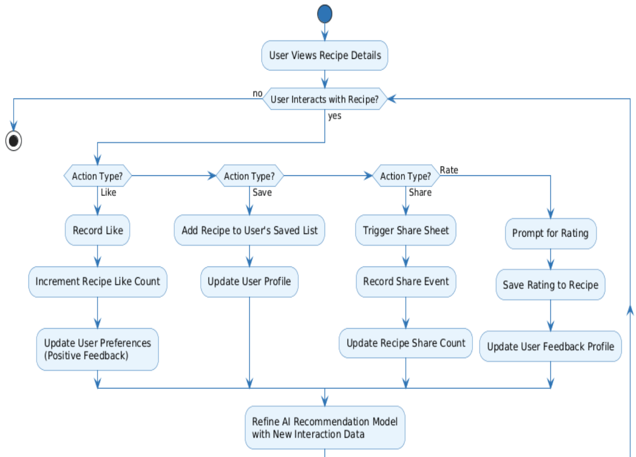
Figure 4.5-4 Activity Diagram: Recipe Interactions
