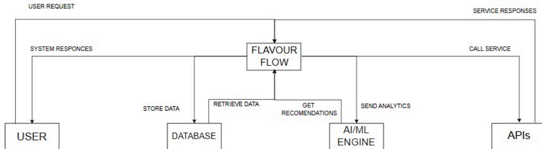
Figure 4.3-1 Data Flow Diagram: Level 0
