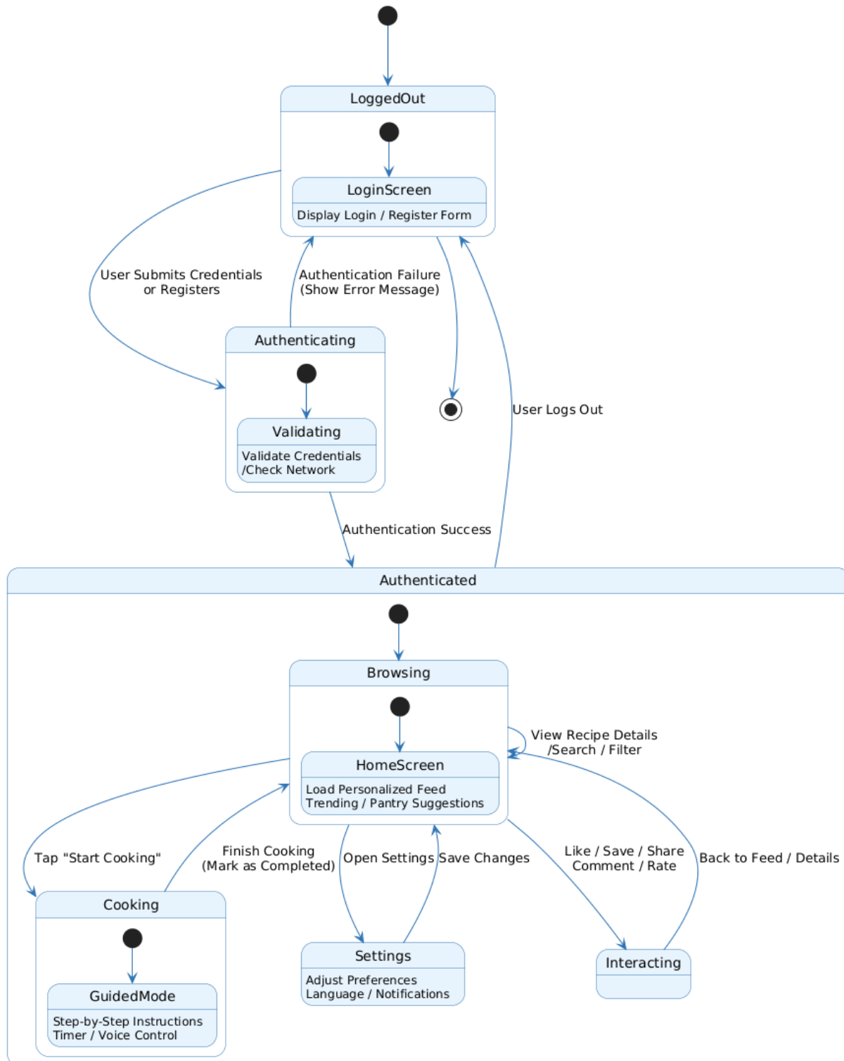
Figure 4.8-1 State Transition Diagram: User State
