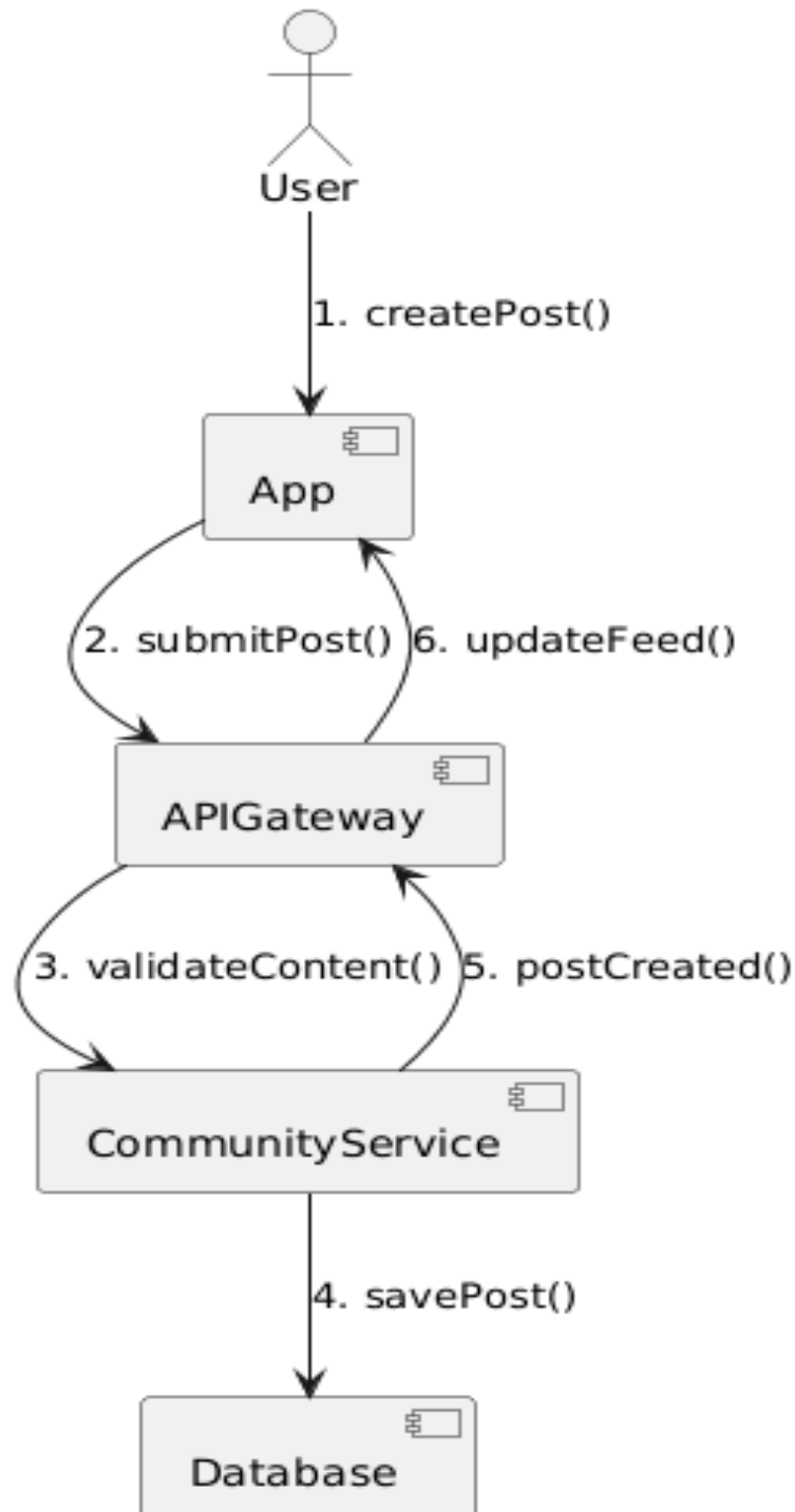
Figure 4.7-3 Collaboration Diagram: Community
