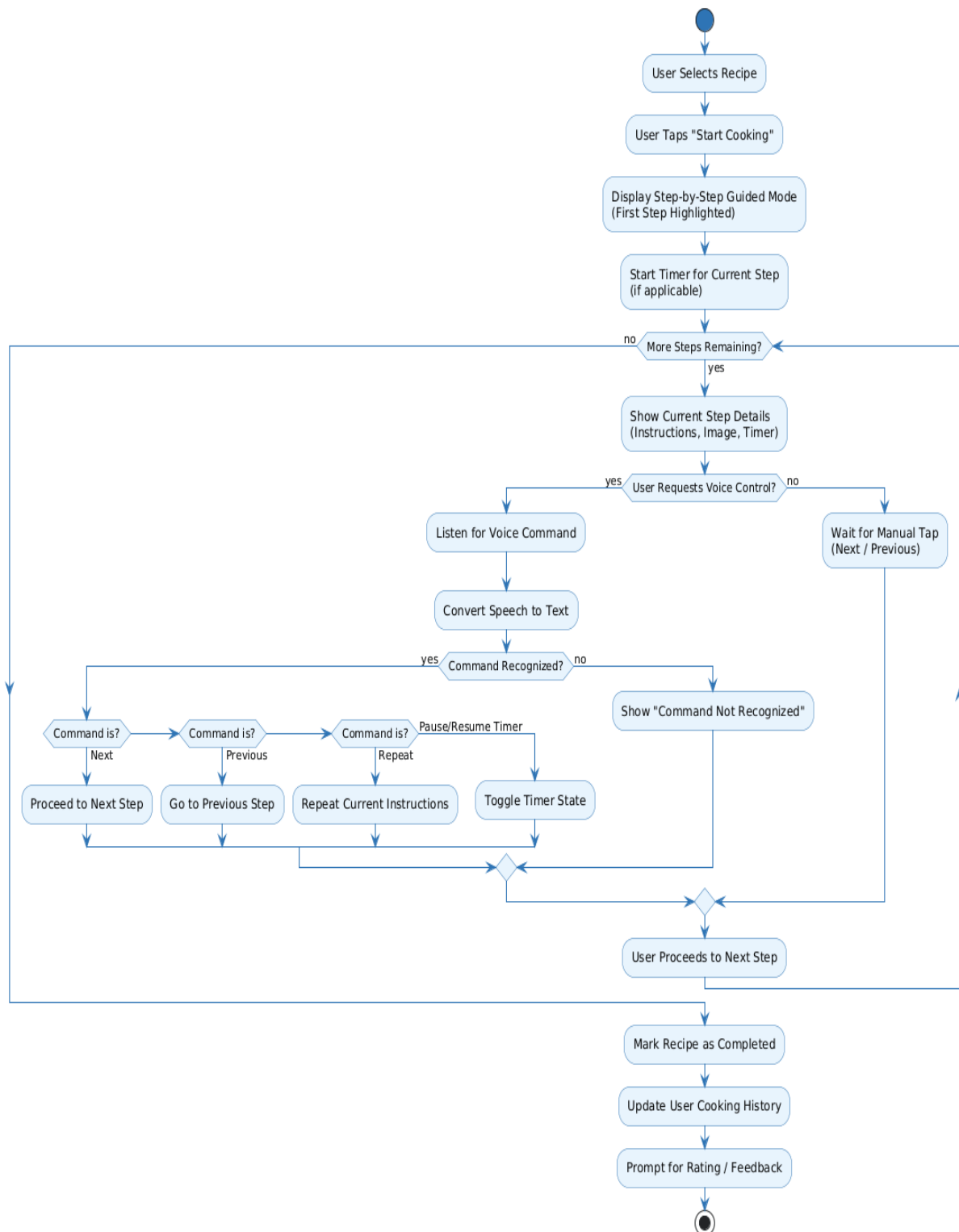
Figure 4.5-10 Activity Diagram: Cooking Assistance
