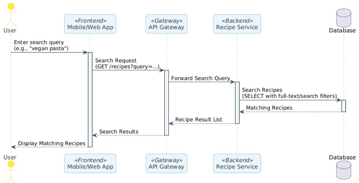
Figure 4.6-5 Sequence Diagram: Recipe Search & Discovery
