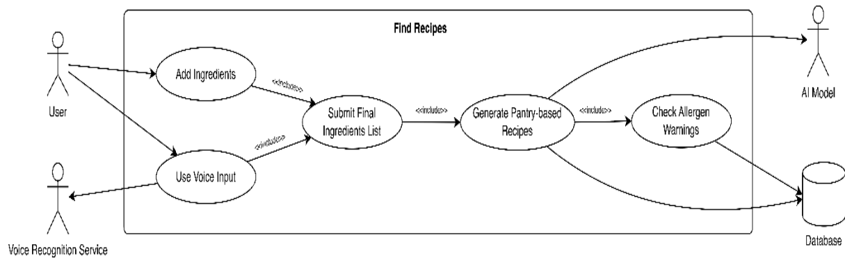
Figure 3.1-9: Find Recipes from Ingredients
