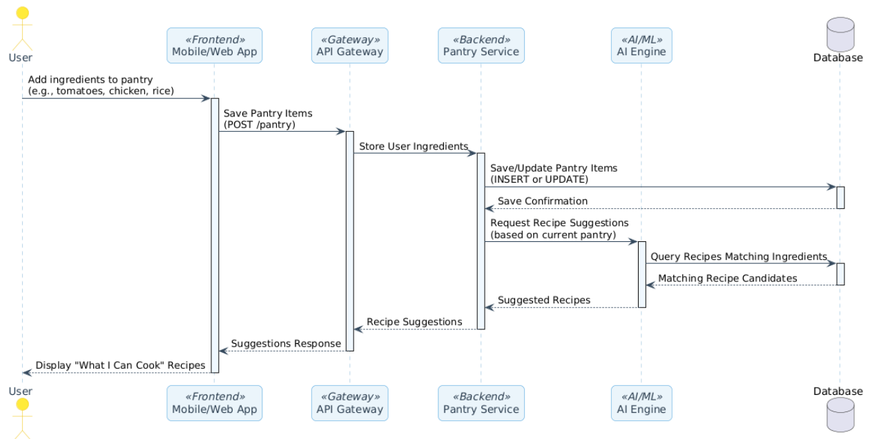
Figure 4.6-9 Sequence Diagram: Smart Pantry & Ingredient Insights
