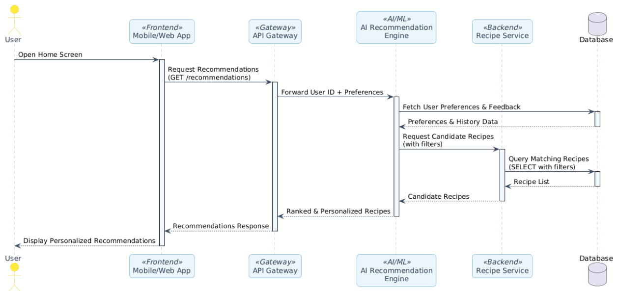
Figure 4.6-3 Sequence Diagram: Meal Recommendation
