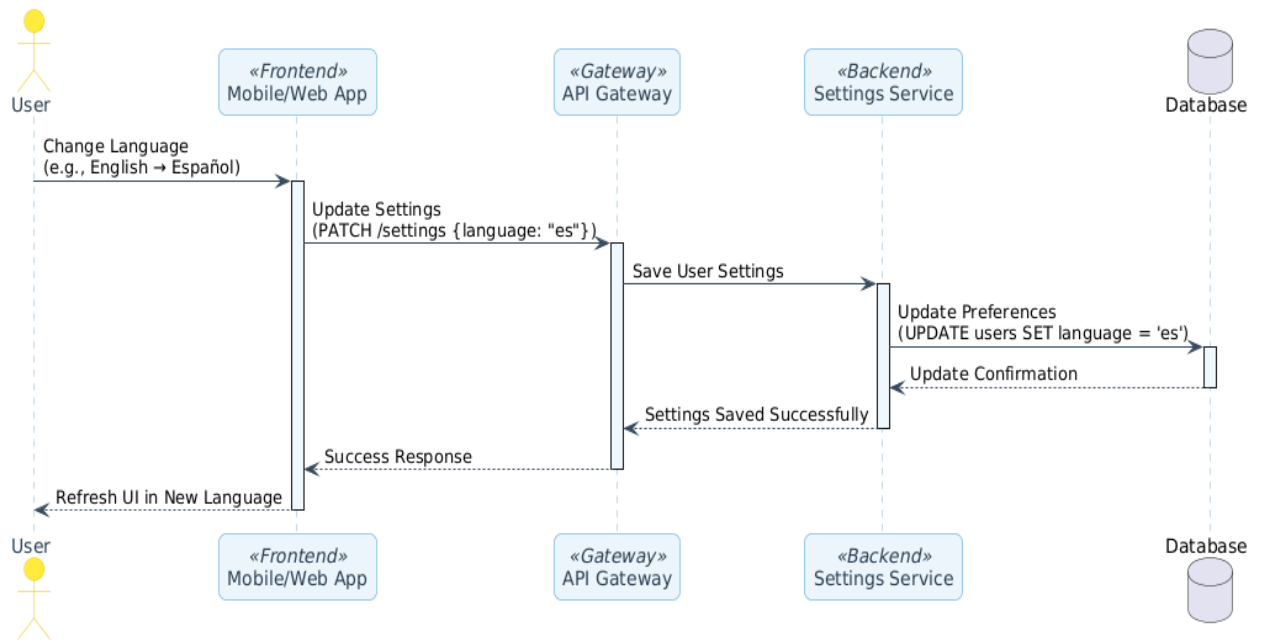
Figure 4.6-12 Sequence Diagram: Manage Application Settings
