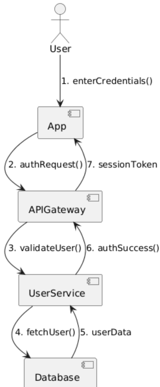
Figure 4.7-1 Collaboration Diagram: Auth
