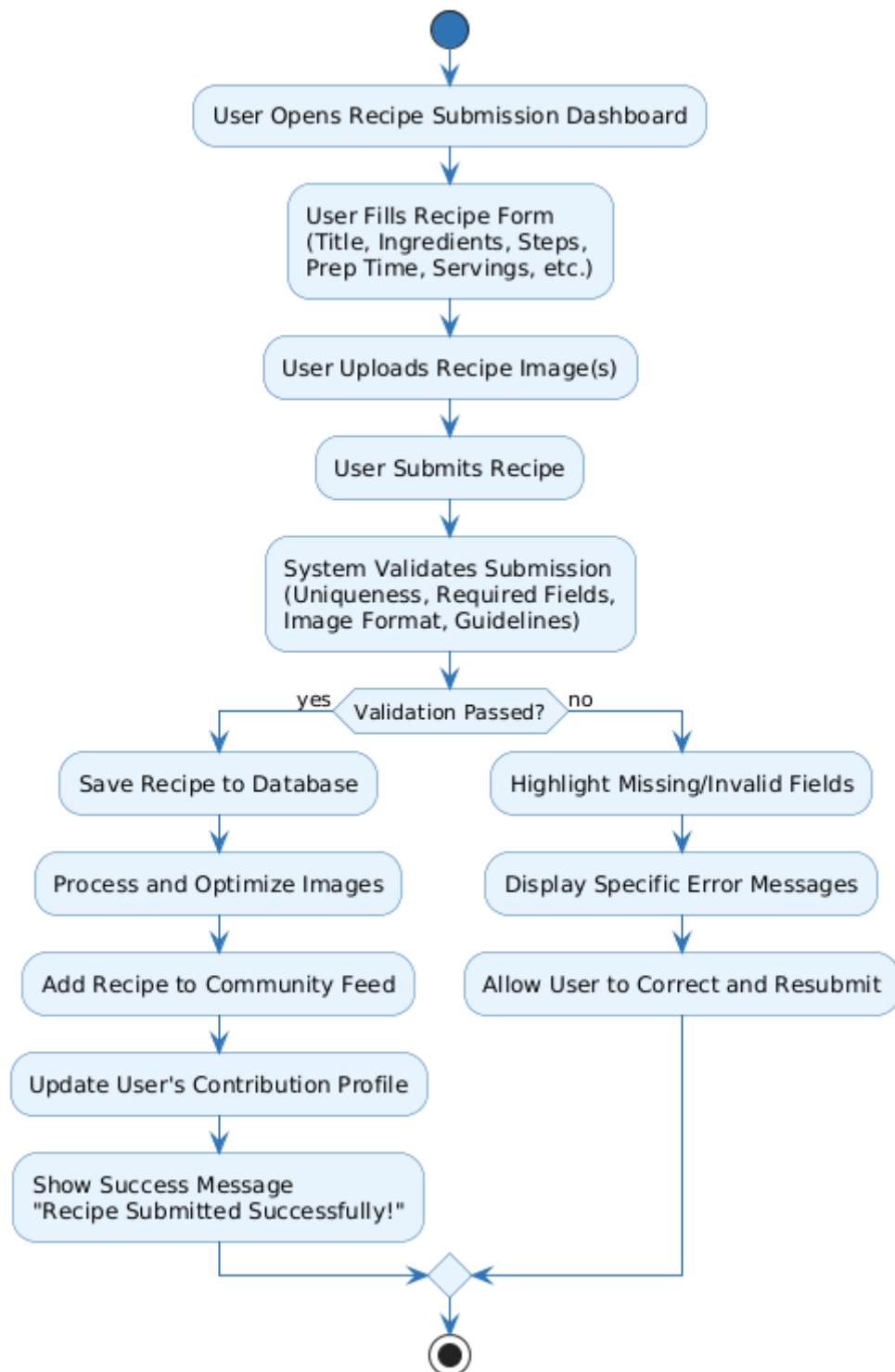
Figure 4.5-7 Activity Diagram: Recipe Upload & Management
