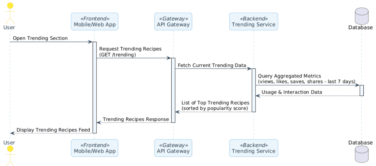
Figure 4.6-11 Sequence Diagram: Trending & Popular Recipes
