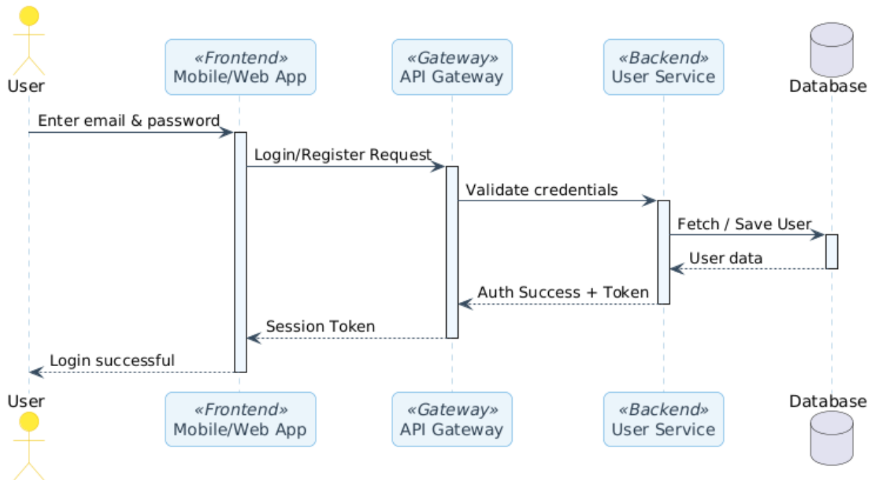
Figure 4.6-1 Sequence Diagram: Account Management
