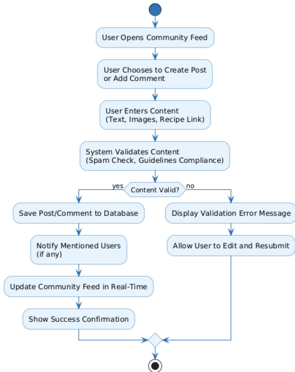
Figure 4.5-6 Activity Diagram: Community Dashboard
