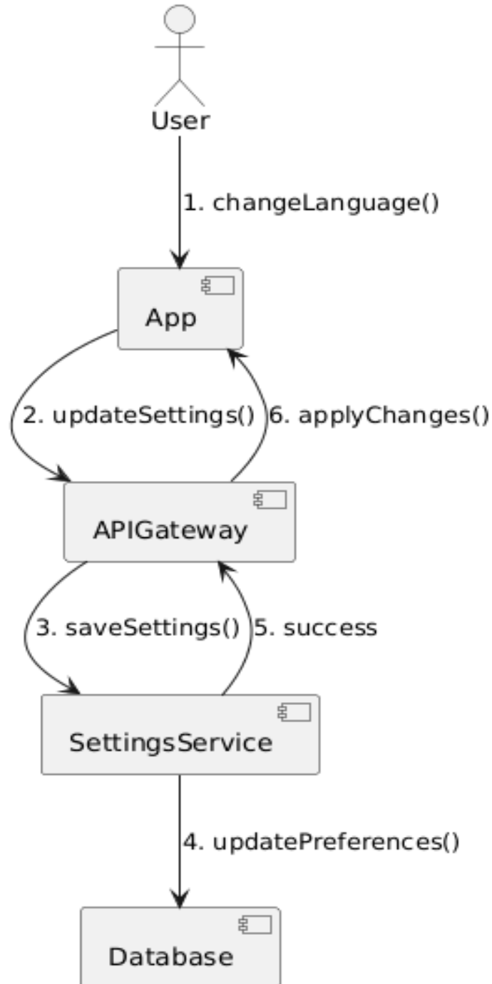
Figure 4.7-7 Collaboration Diagram: Application Settings & Localization
