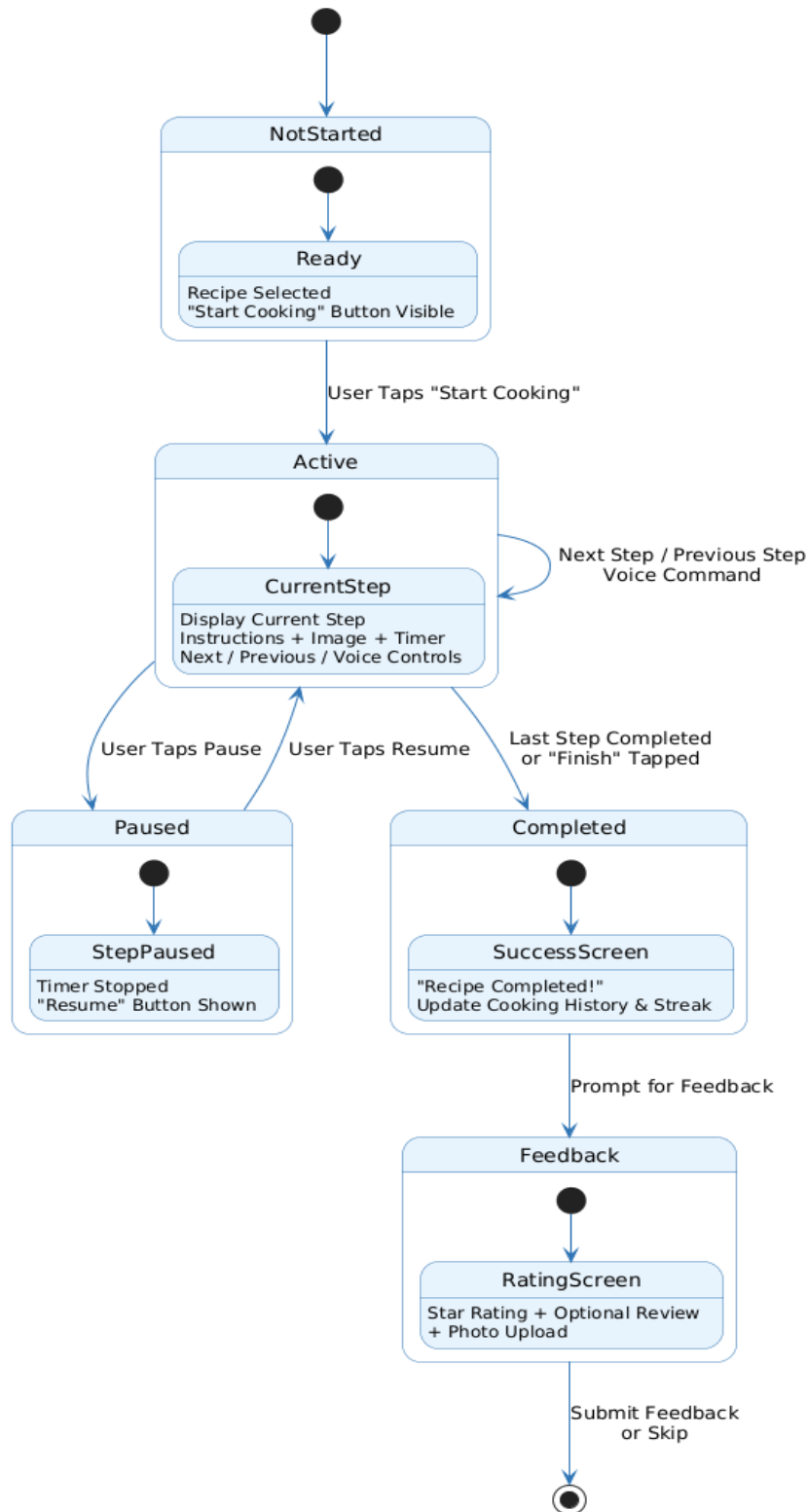
Figure 4.8-2 State Transition Diagram: Cooking Session
