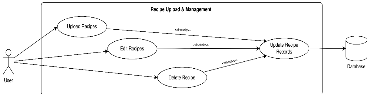
Figure 3.1-7: Recipe Upload and Management
