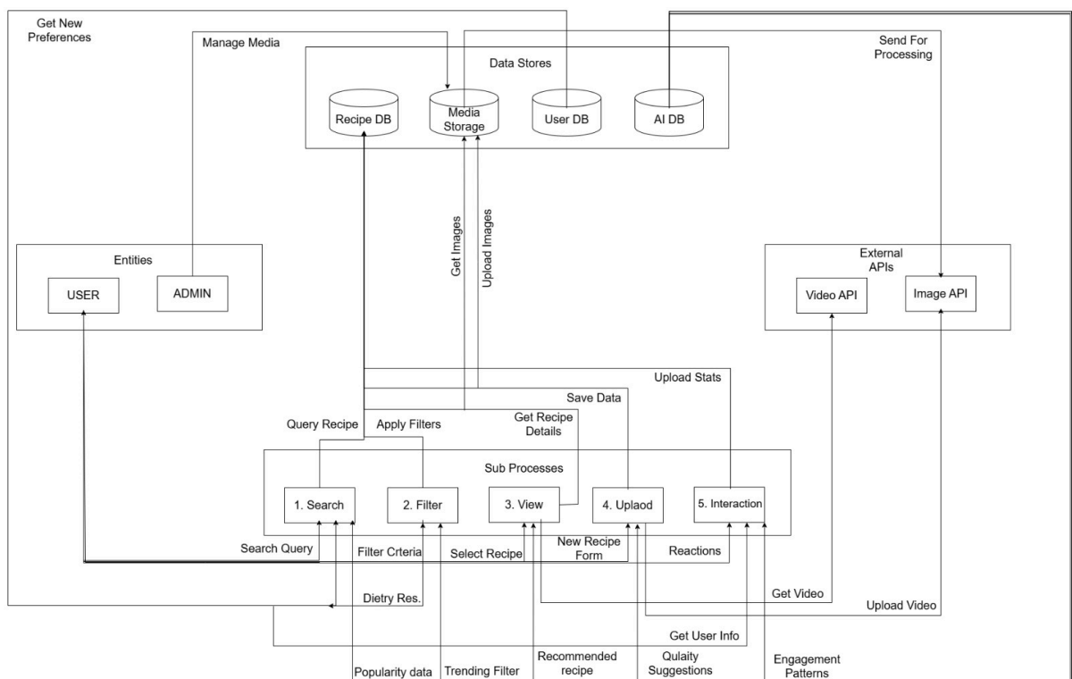
Figure 4.3-2 Data Flow Diagram: Level 1
