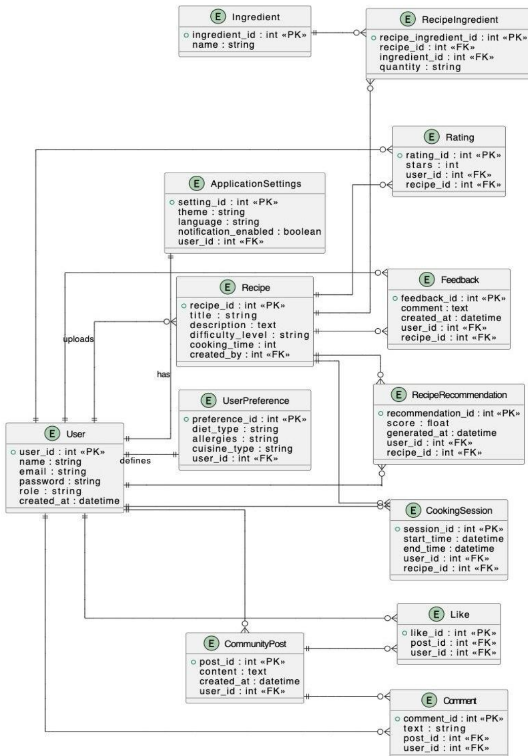
Figure 4.2-1 ERD with data dictionary
