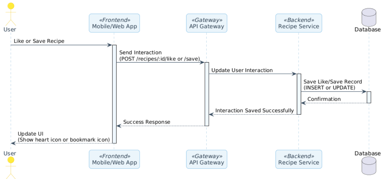
Figure 4.6-4 Sequence Diagram: Recipe Interactions
