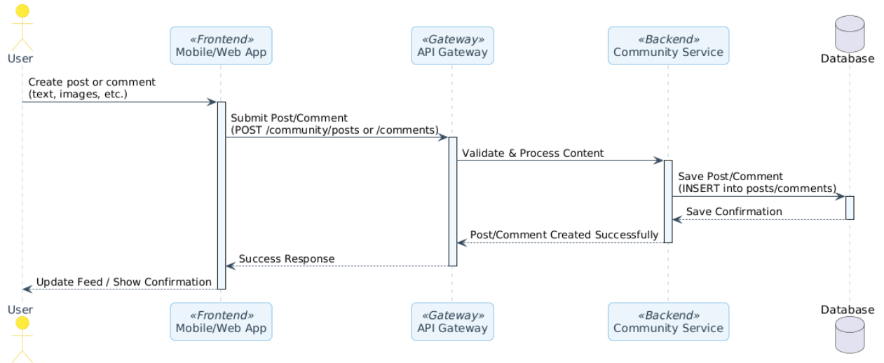
Figure 4.6-6 Sequence Diagram: Community Dashboard
