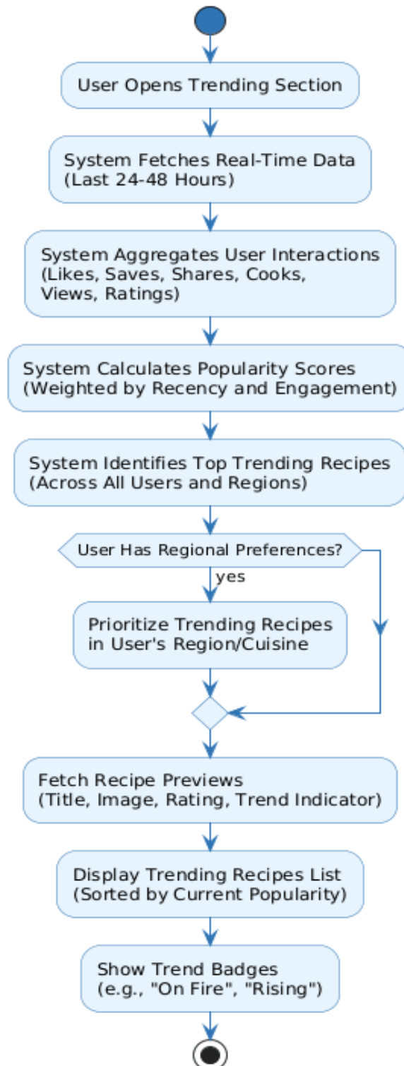
Figure 4.5-11 Activity Diagram: Trending & Popular Recipes
