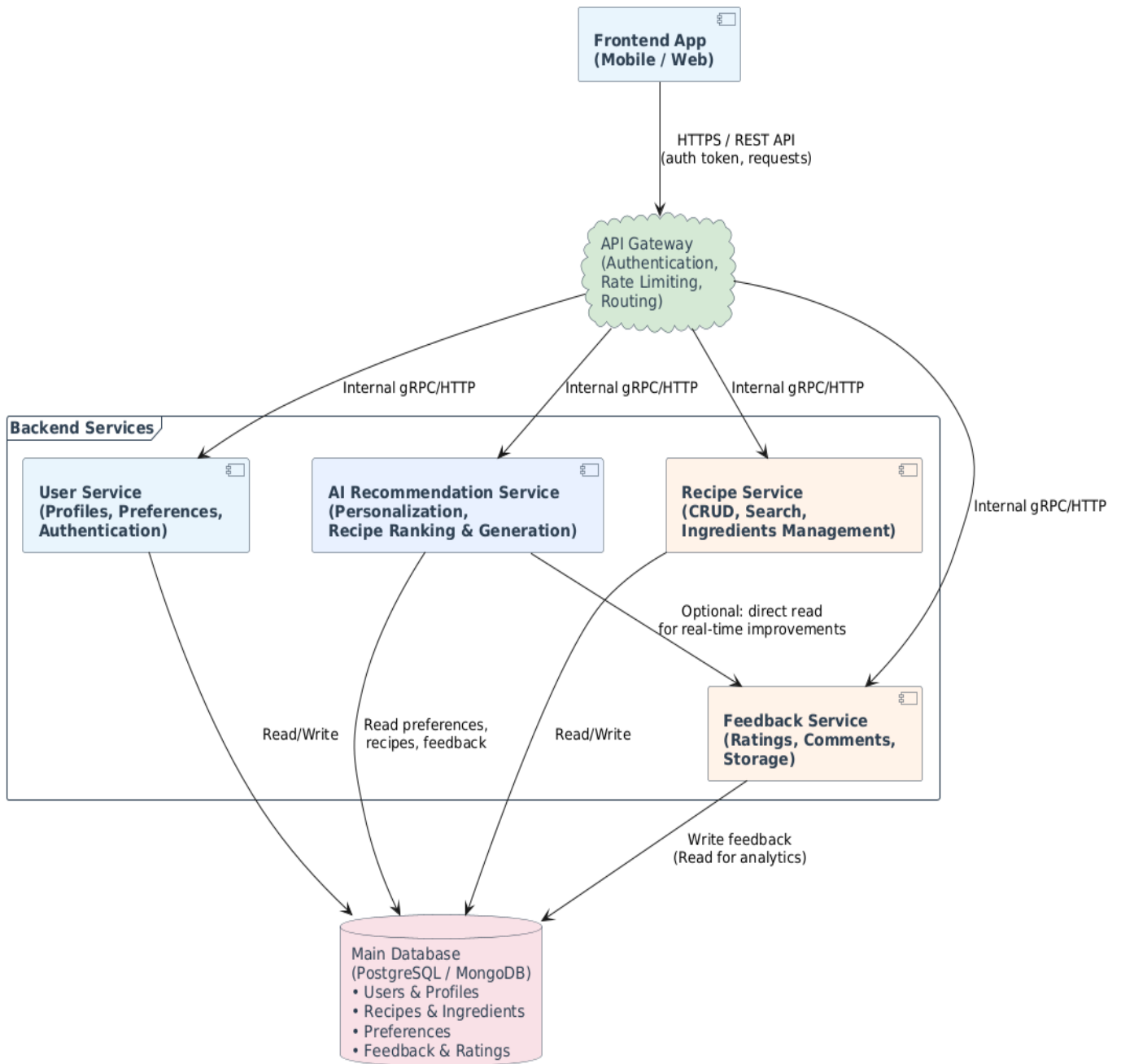
Figure 4.9-1 Component Diagram
