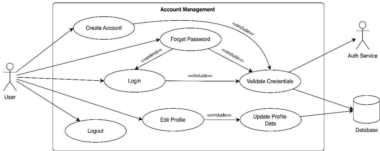
Figure 3.1-1: Account Management
