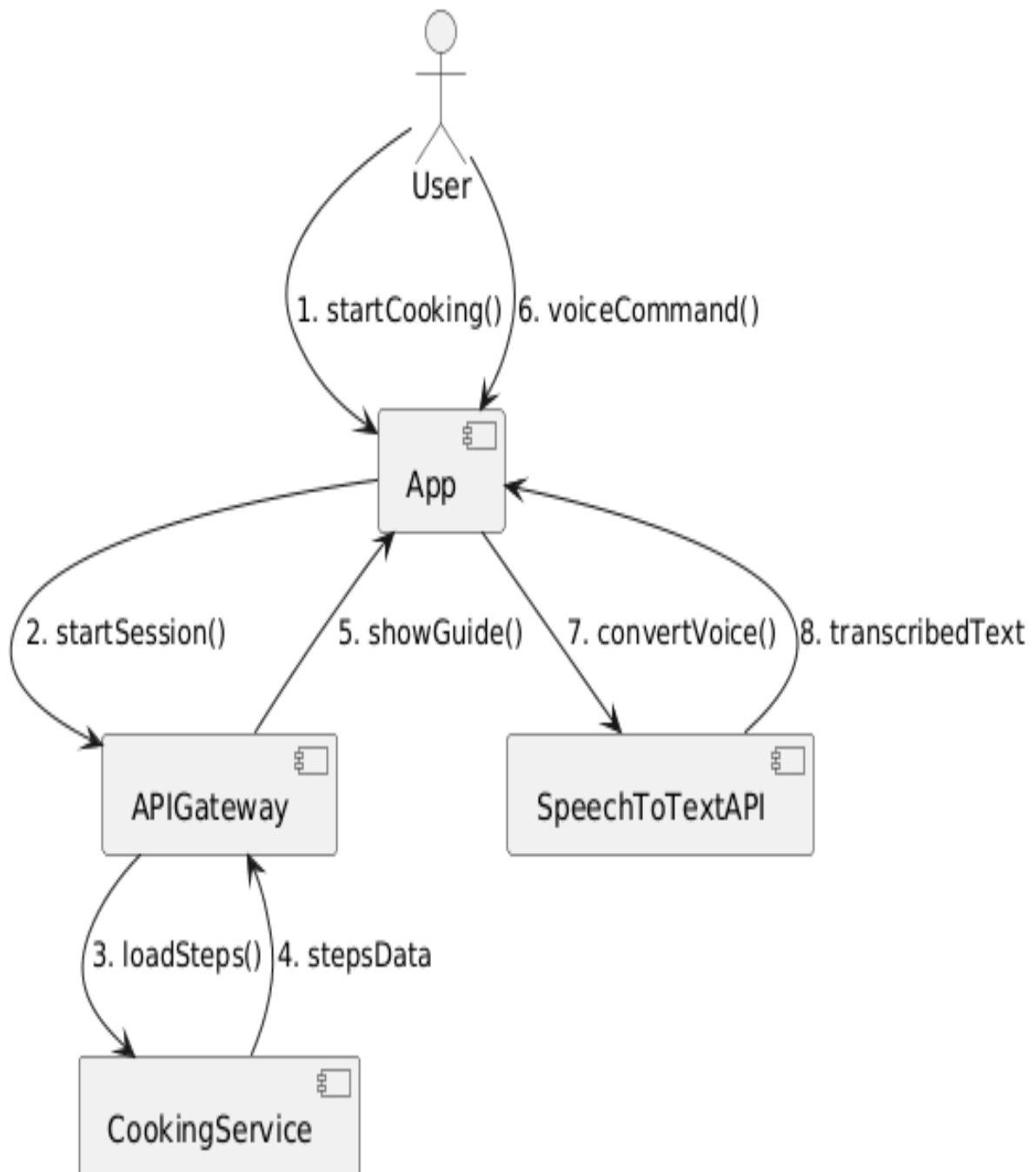
Figure 4.7-6 Collaboration Diagram: Cooking Assistance
