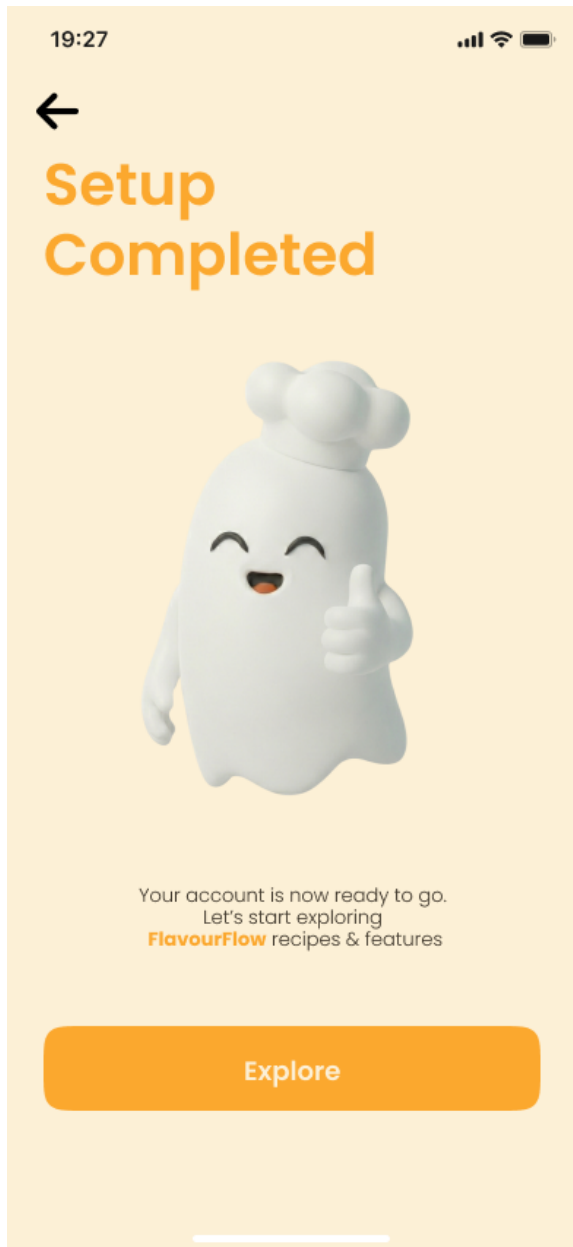
Figure 5.1-15 Setup Completion
