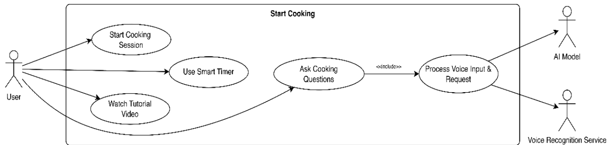
Figure 3.1-10: Start Cooking
