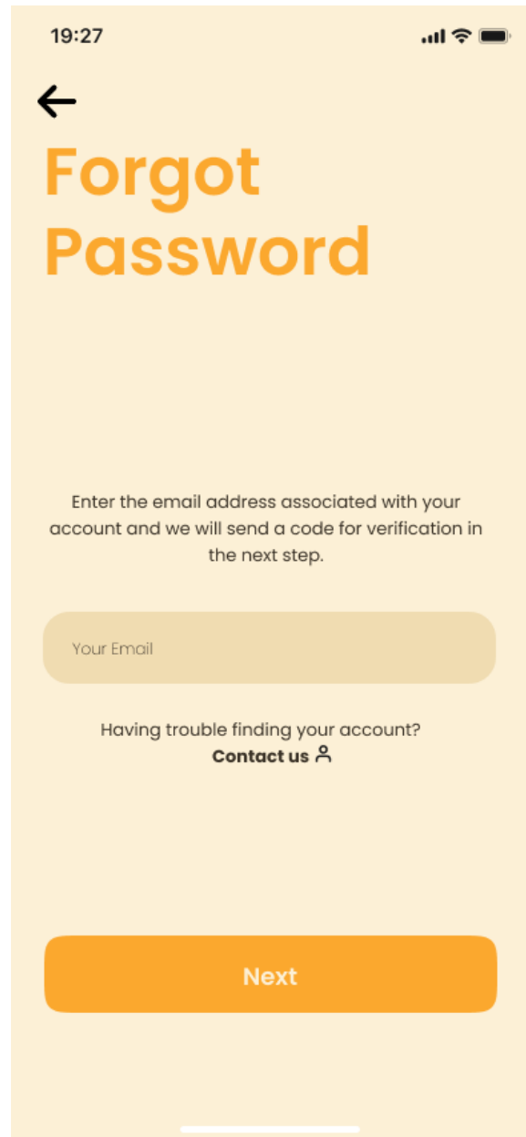
Figure 5.1-3 Forget Password
