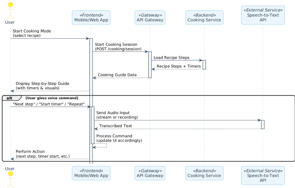
Figure 4.6-10 Sequence Diagram: Cooking Assistance
