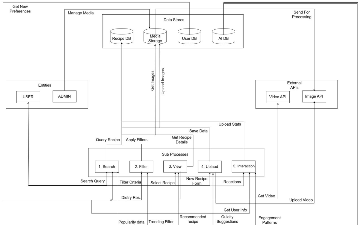
Figure 4.3-3 Data Flow Diagram: Level 2
