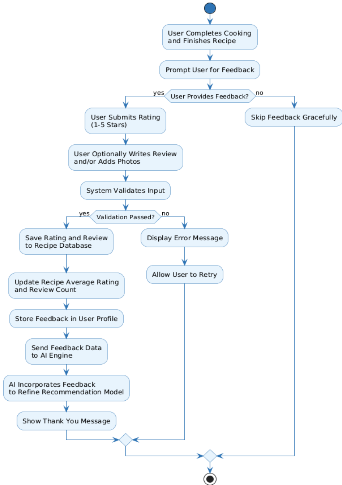
Figure 4.5-8 Activity Diagram: Feedback & Rating
