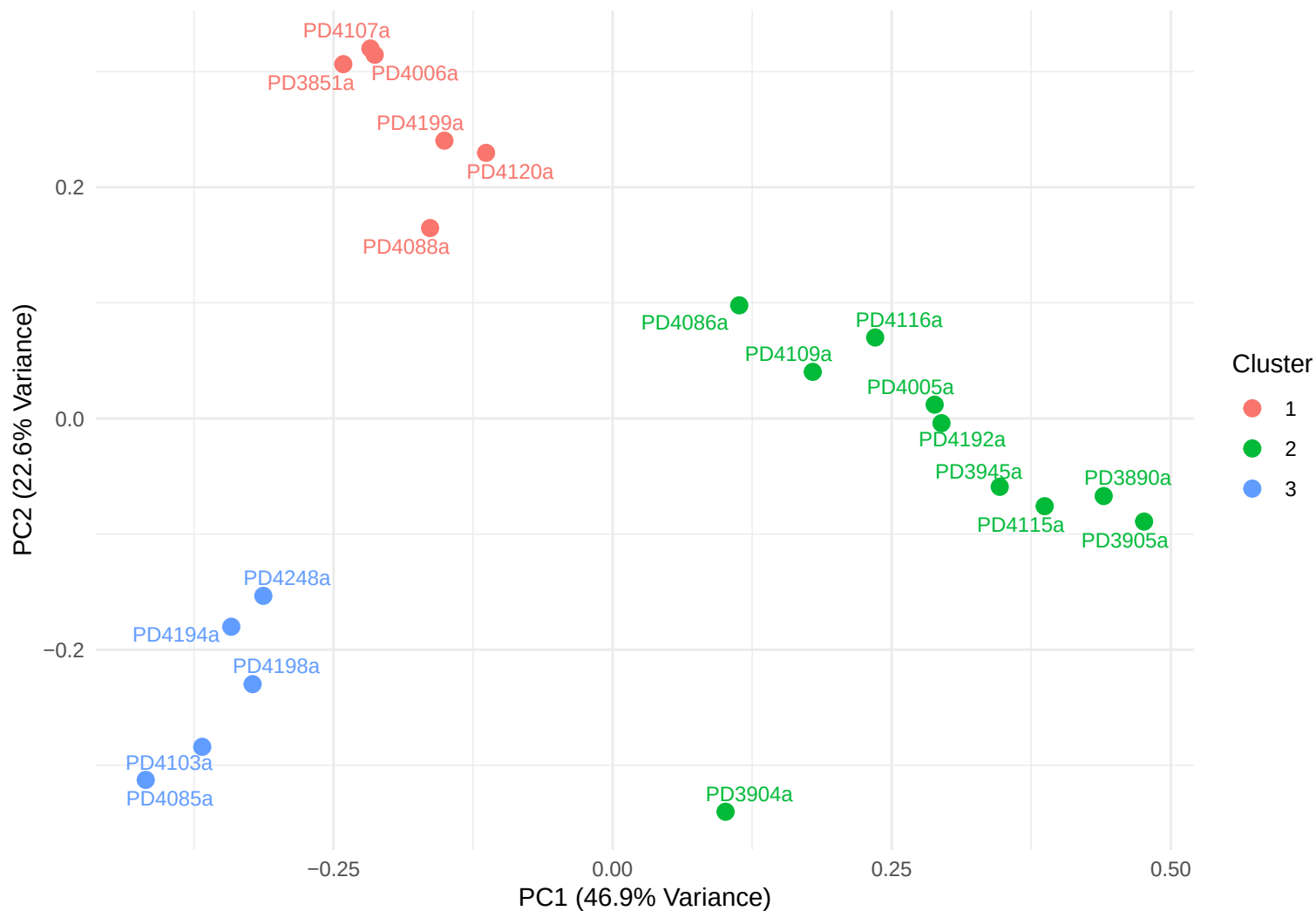
PCA of Mutation Signatures Colored by K-Means Clusters (k = 3 )
