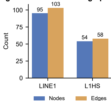
c Smoke-tested graph queries
