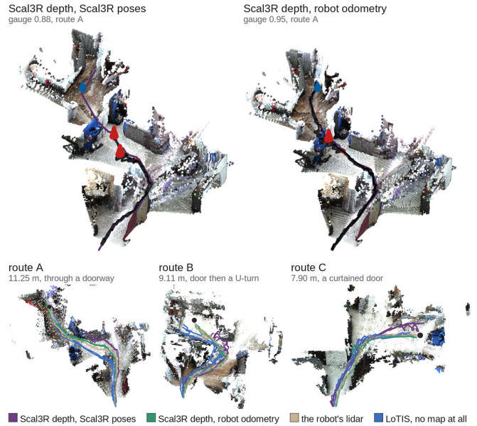
Fig. 5: Top, route A from the same Scal3R depth at two sets of poses: plum the plan, black every driven run, red a collision, a pin where a run did not finish, blue the walk’s end. Bottom, the three routes from above on the robot’s lidar, with all 34 runs, one colour per case.
