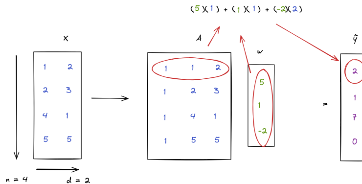
Figure 6: Example of a multiple linear regression.
