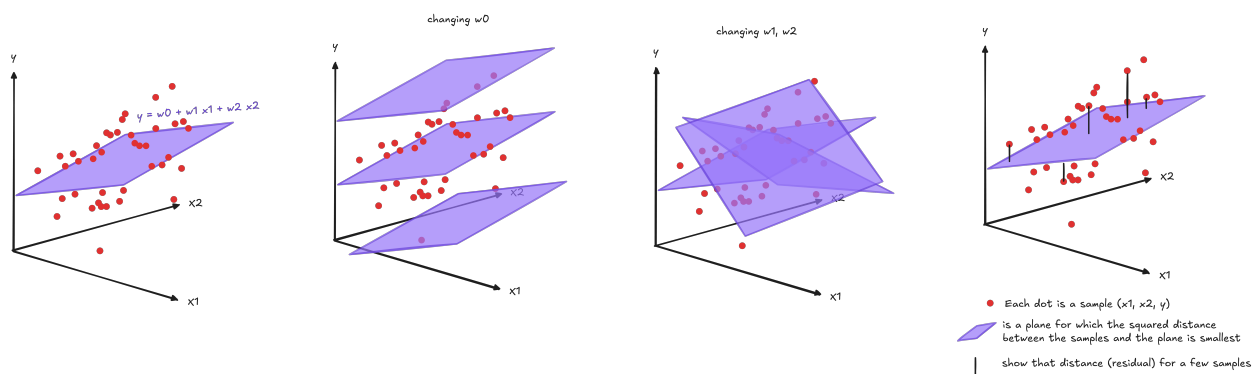
Figure 7: In 2D, the least squares regression is now a plane. In higher d , it's a hyperplane.
