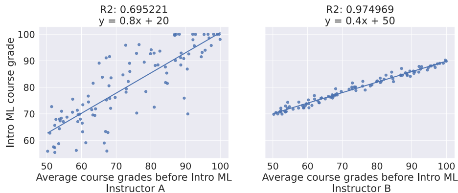
Figure 5: Predicting students’ grades in Intro ML, for two different sections.
