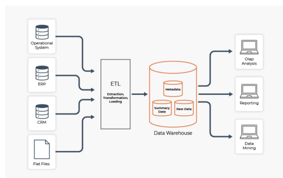
Figure 3.3: Data Warehouse Architecture.
