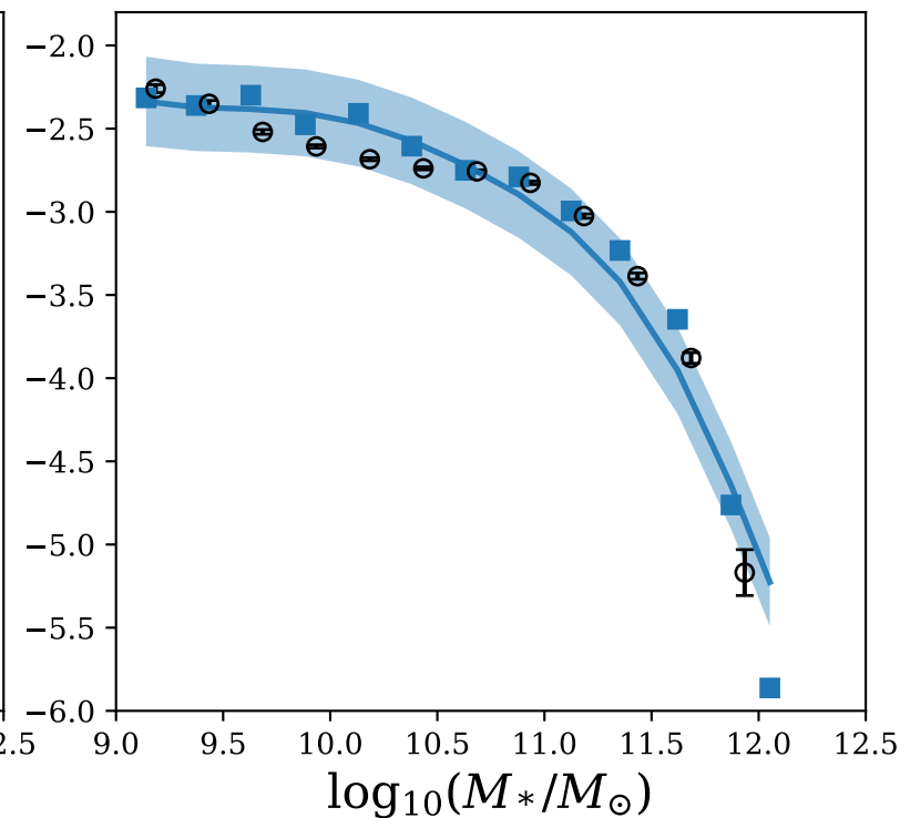
Simulation fiducial
