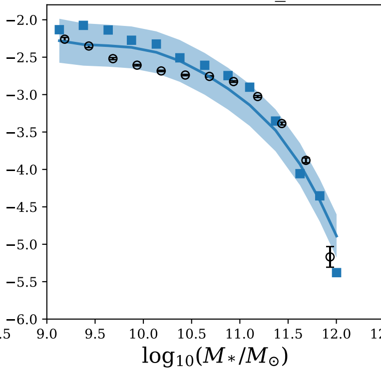
Simulation LH_12
