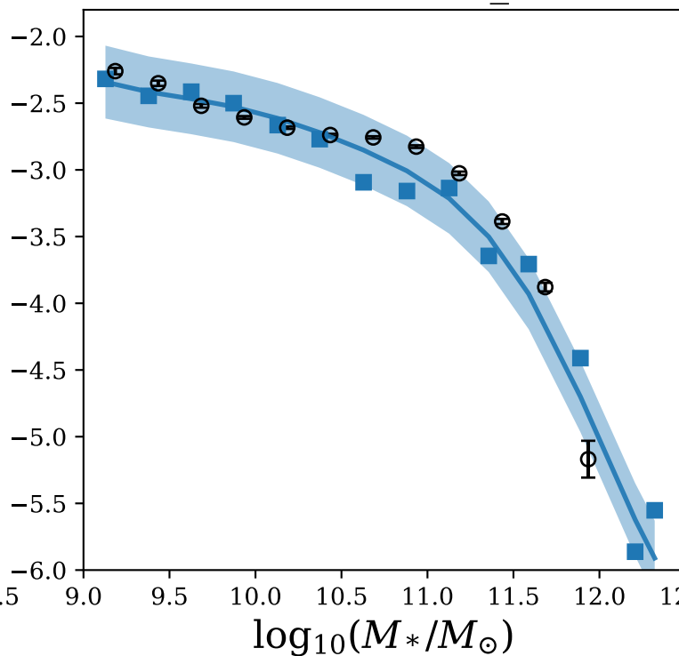
Simulation LH_28
