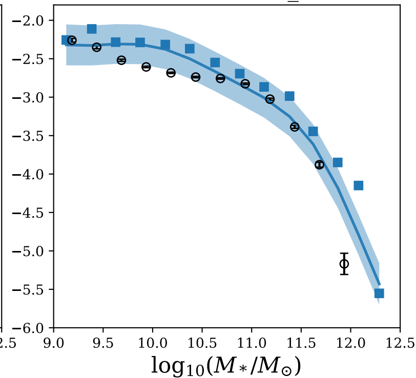
Simulation LH_16
