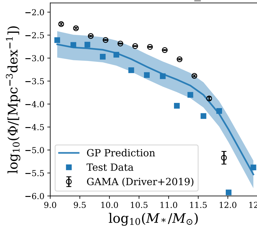
Simulation LH_8
