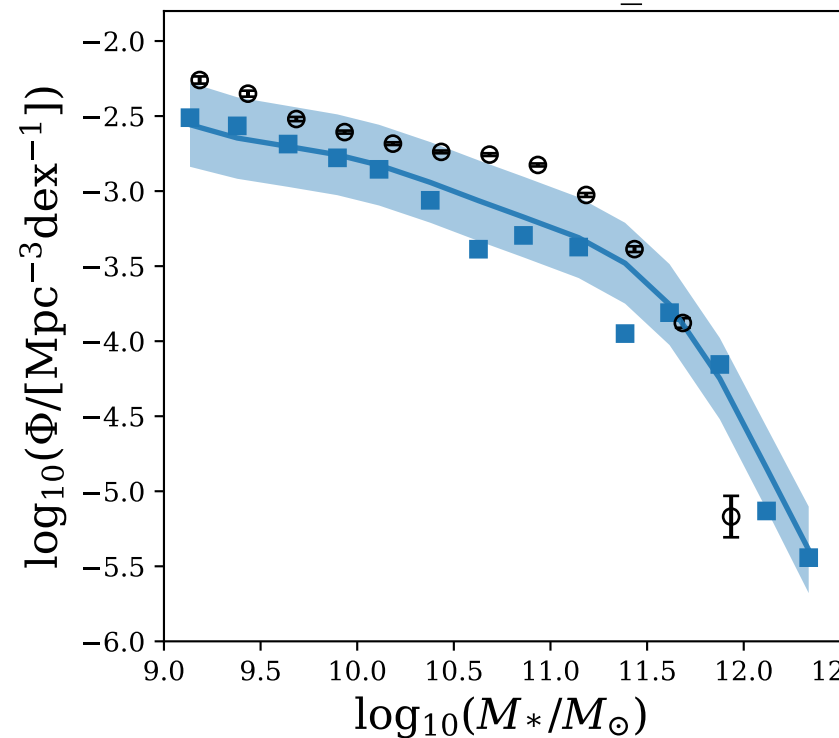
Simulation LH_23
