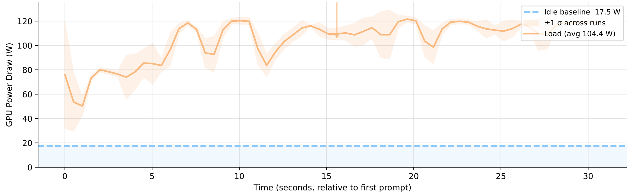
GPU Power Timeline — deepseek-r1:1.5b (off) (3 runs averaged)
