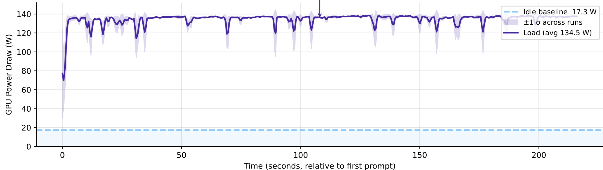
GPU Power Timeline — deepseek-r1:7b (on) (3 runs averaged) Idle: 17.3 W | Load avg: 134.5 W | \Delta = +117.2 W
