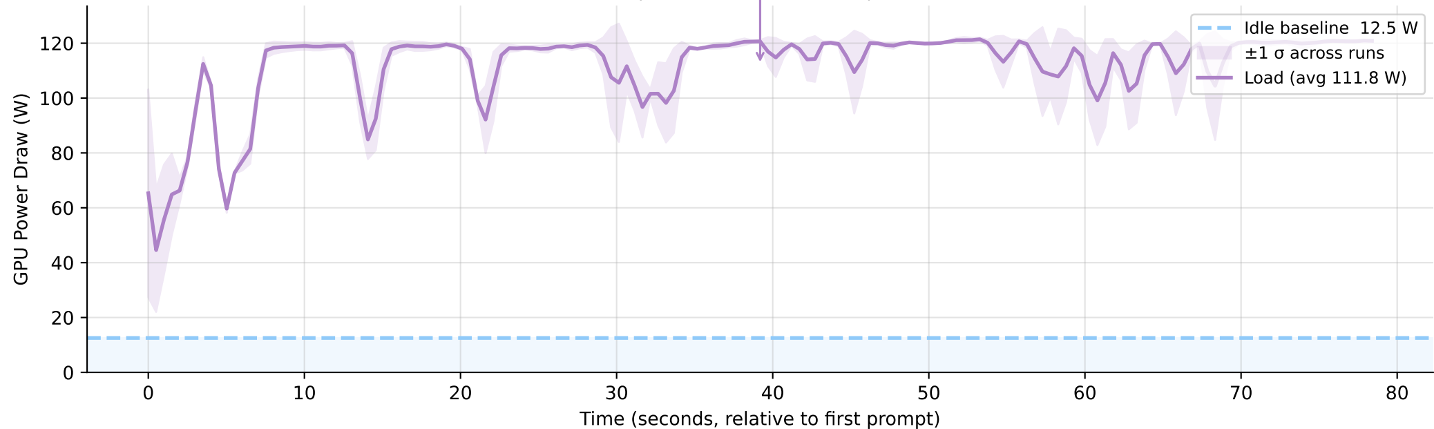
GPU Power Timeline — gemma4:e2b (off) (3 runs averaged) Idle: 12.5 W | Load avg: 111.8 W | \Delta = +99.2 W
