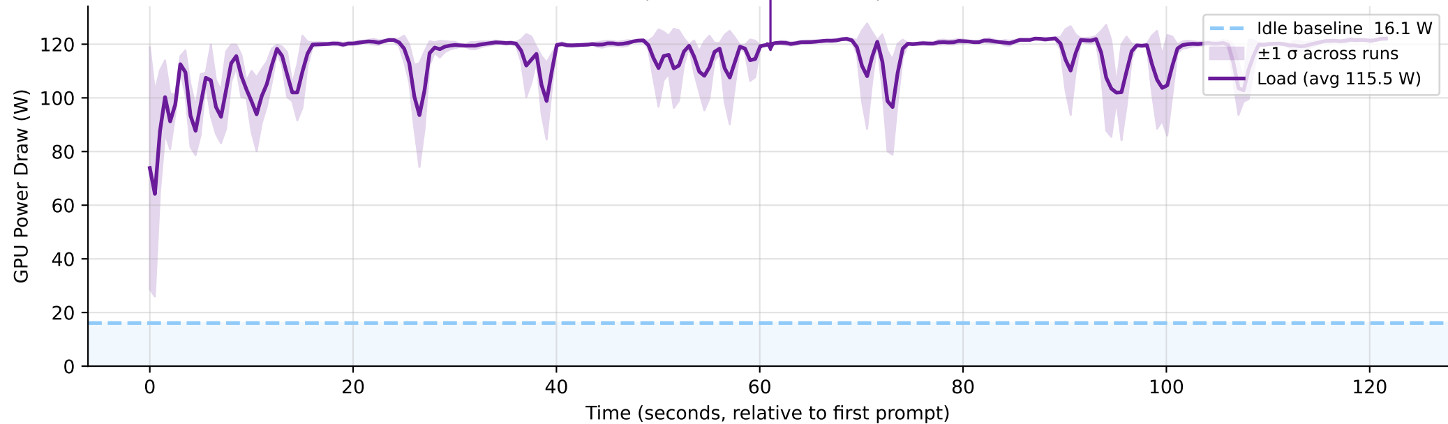
GPU Power Timeline — gemma4:e2b (on) (3 runs averaged) Idle: 16.1 W | Load avg: 115.5 W | \Delta = +99.5 W
