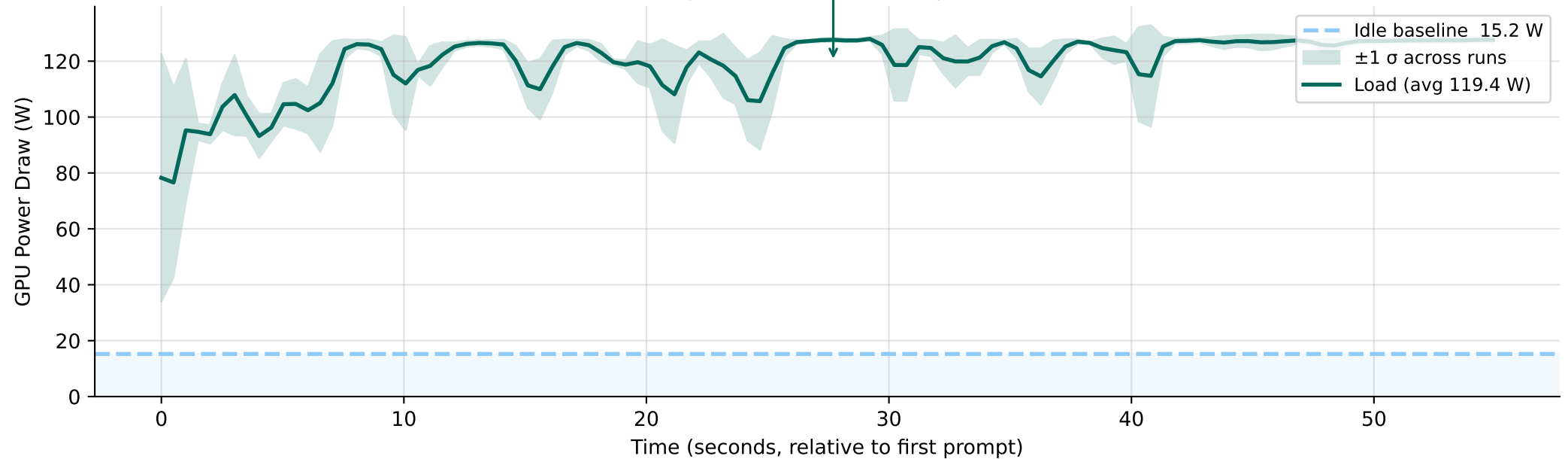
GPU Power Timeline — granite3.1-dense:2b (3 runs averaged) Idle: 15.2 W | Load avg: 119.4 W | \Delta = +104.2 W
