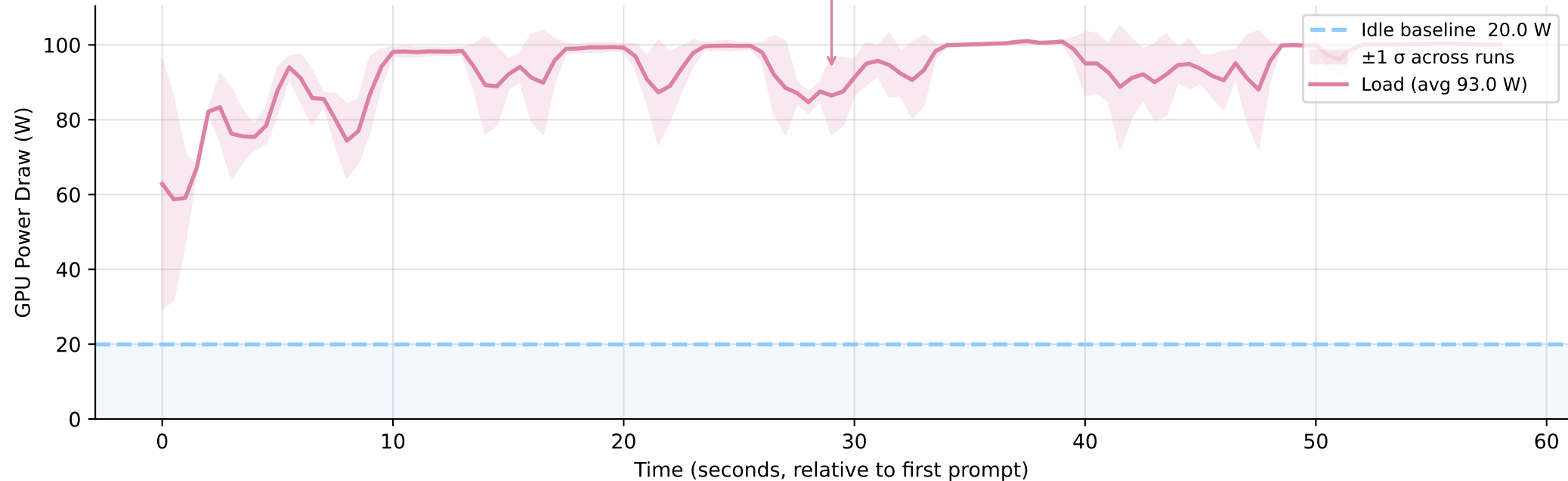
GPU Power Timeline — qwen3.5.0.8b (off) (3 runs averaged) Idle: 20.0 W | Load avg: 93.0 W | \Delta = +73.1 W
