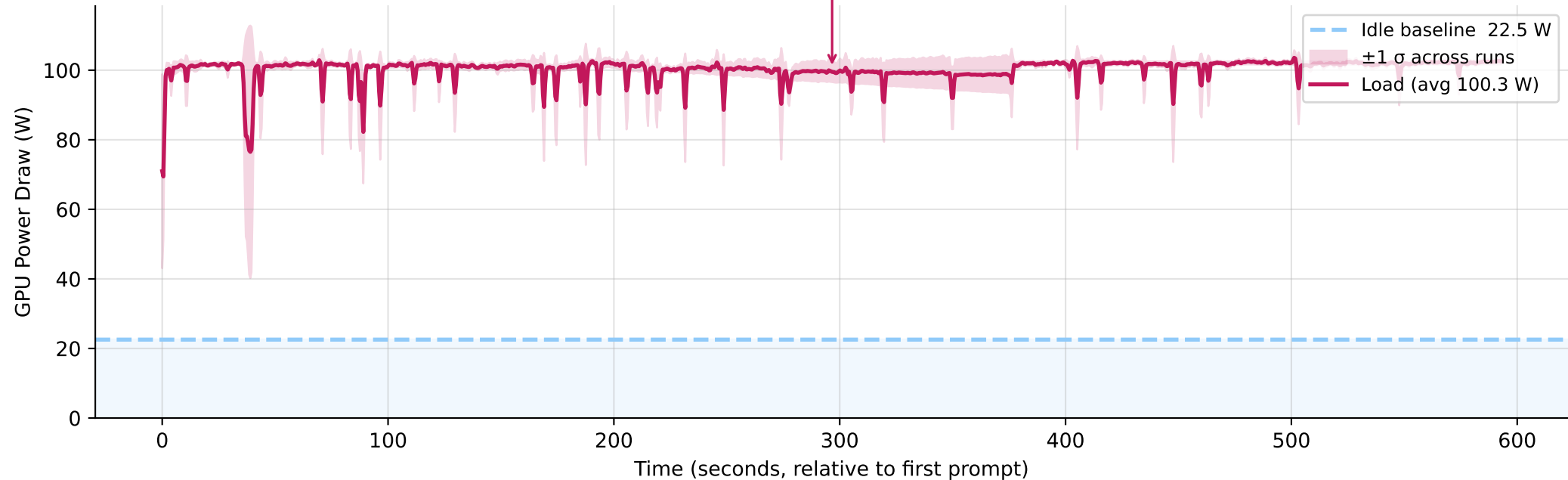
GPU Power Timeline — qwen3 72B (on) (3 runs averaged) Idle: 22.5 W | Load avg: 100.3 W | \Delta = +77.8 W
