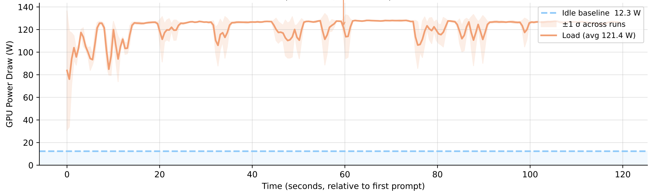
GPU Power Timeline — qwen3.5:4b (off) (3 runs averaged) Idle: 12.3 W | Load avg: 121.4 W | \Delta = +109.1 W
