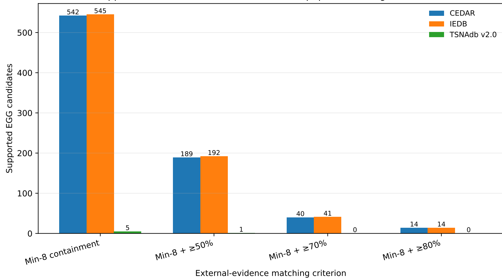
Supported EGG candidates retained under peptide-coverage thresholds
