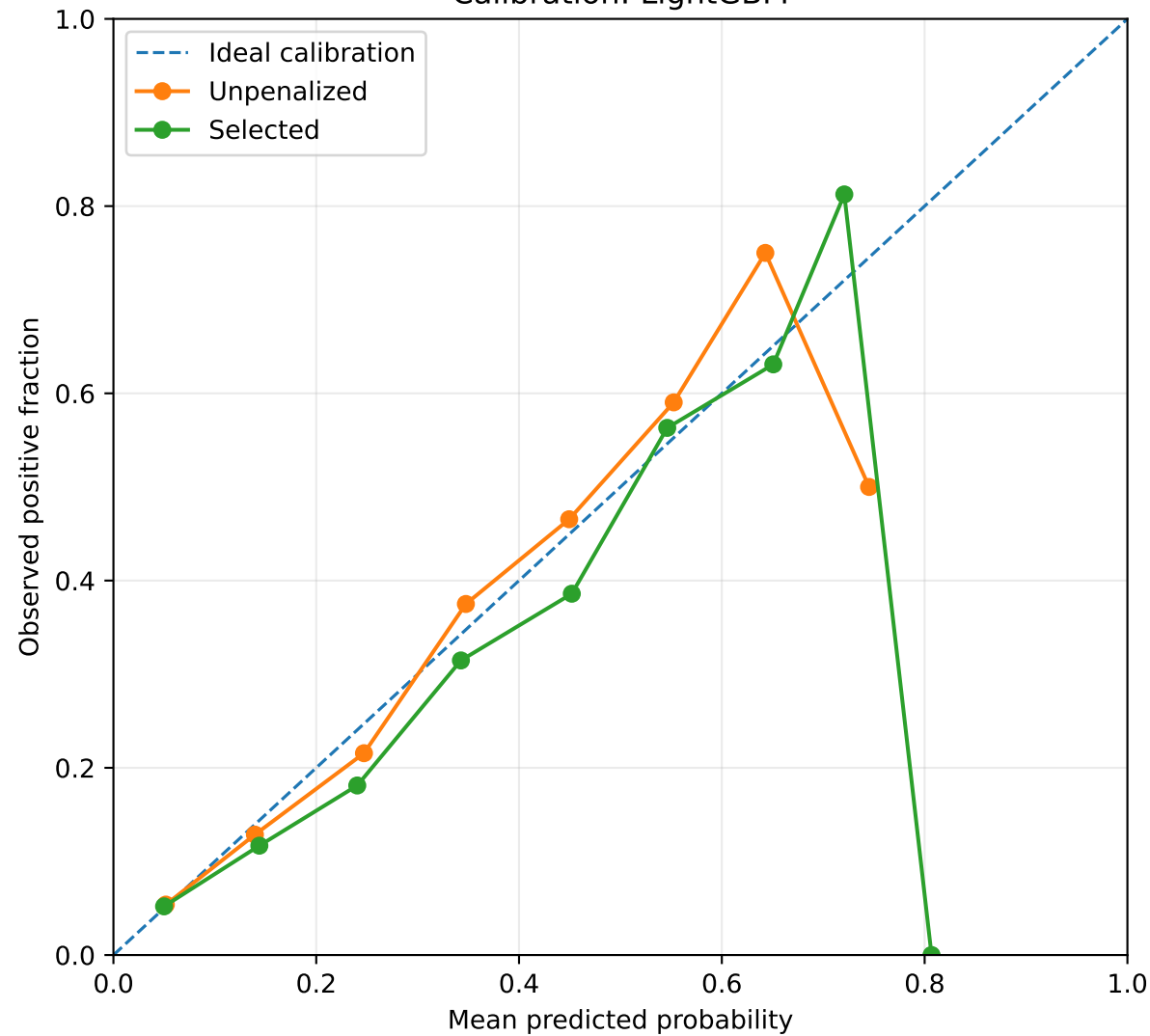
Calibration: LightGBM
